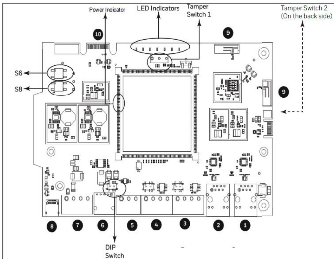
PCB Layout
