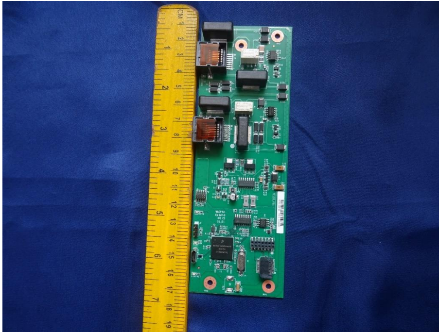
Photo 11: Pot PCB dimensional View
