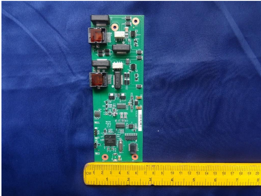
Photo 12: Pot PCB dimensional View
