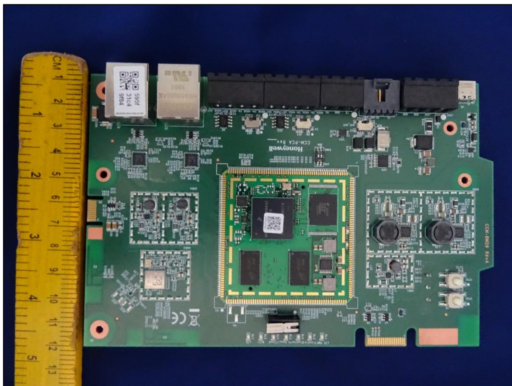
Figure 4: Dimensional view of Anchor
