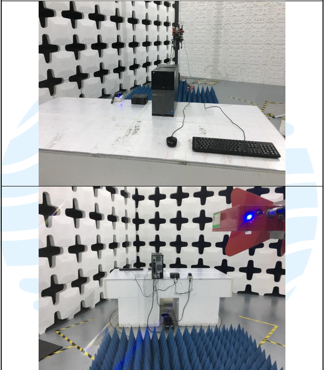
Radiated emission Test Setup (Above 1 GHz) _TM1
