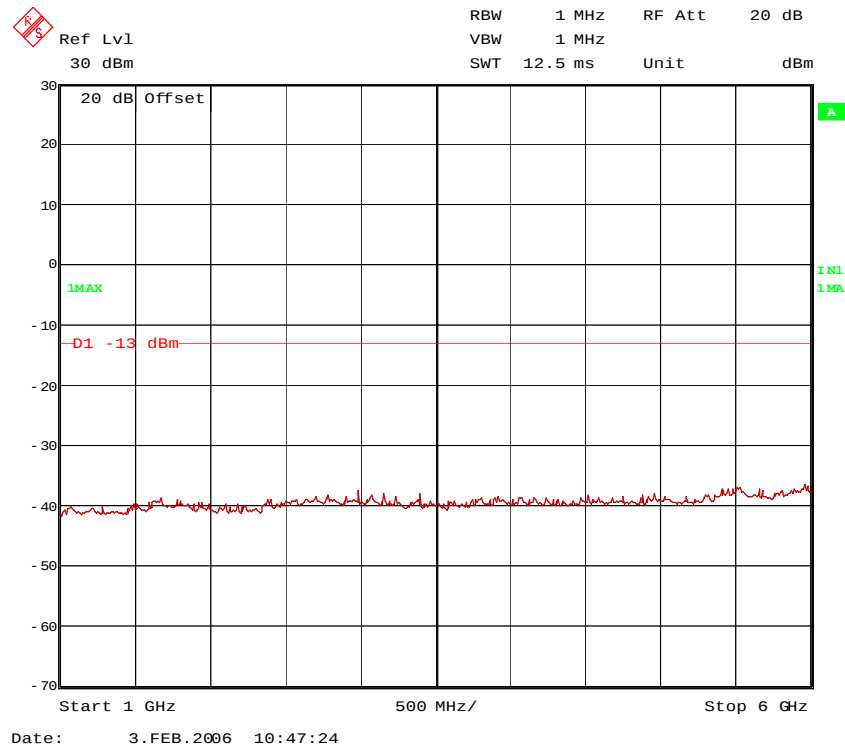
52367c470tx4.wmf: 1 GHz to 6 GHz
