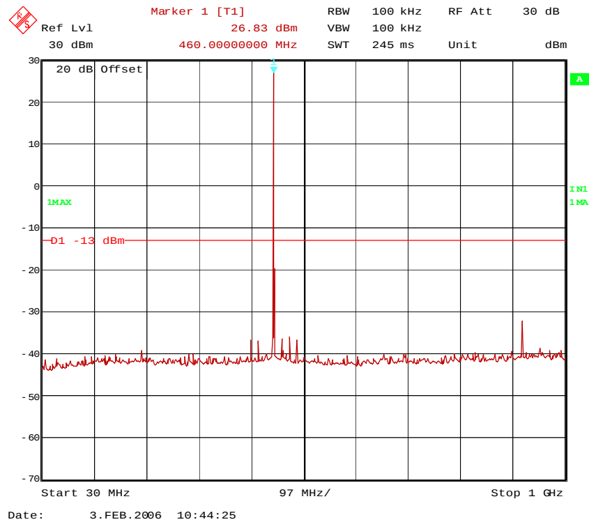
52367c460tx1.wmf: 30 MHz to 1 GHz
