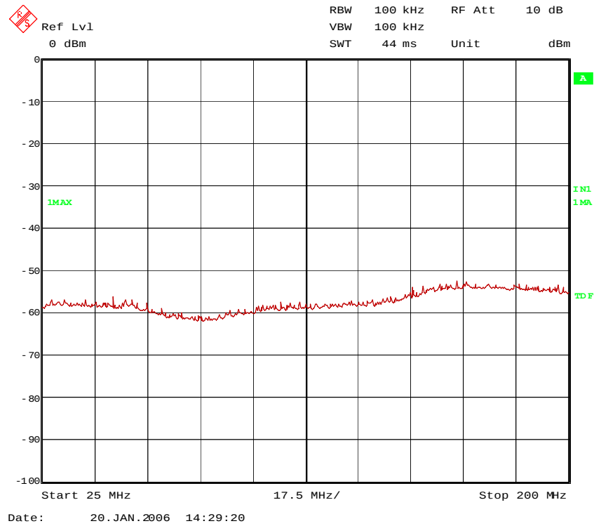
52367_470tx1.wmf: 25 MHz to 200 MHz
