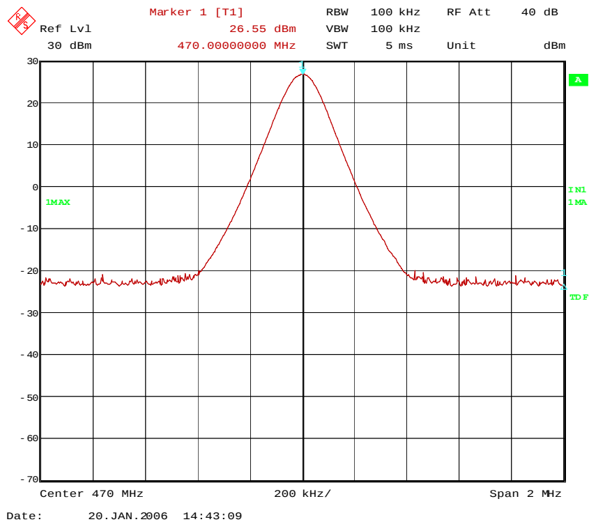
52367_470pwr.wmf: Radiated Transmitter Output Power
