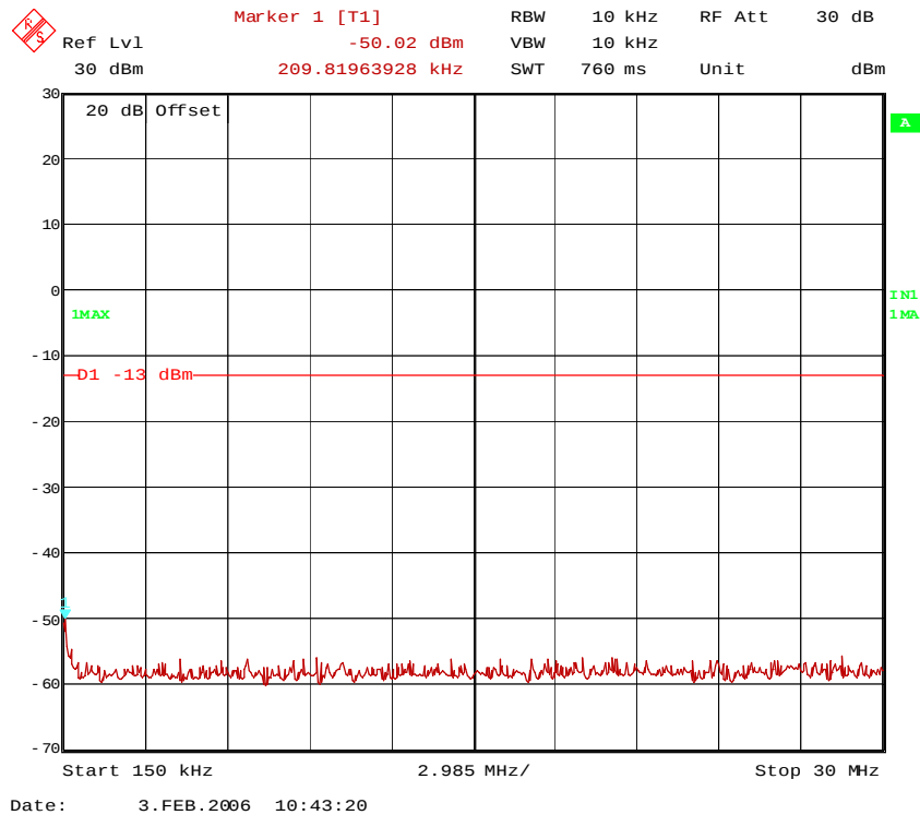
52367c470tx2.wmf: 150 kHz to 30 MHz
