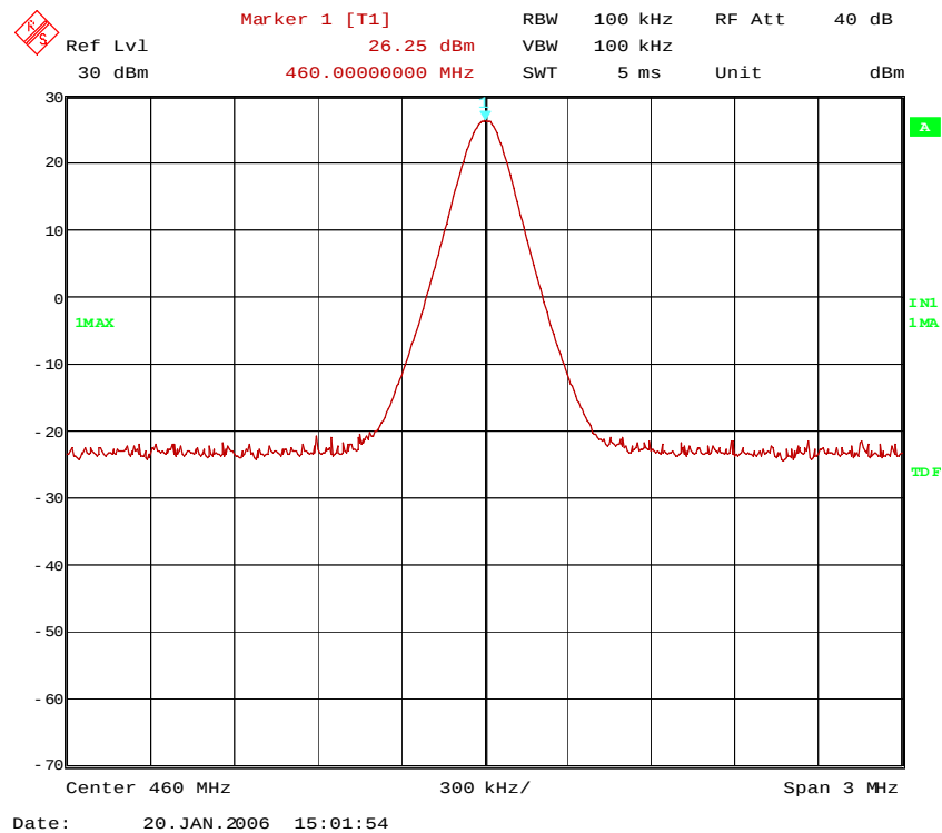
52367_460pwr.wmf: Radiated Transmitter Output Power
