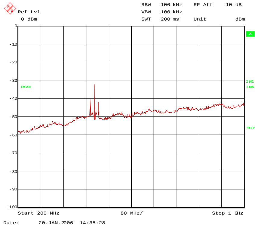
52367_470tx2wmf: 200 MHz to 1000 MHz
