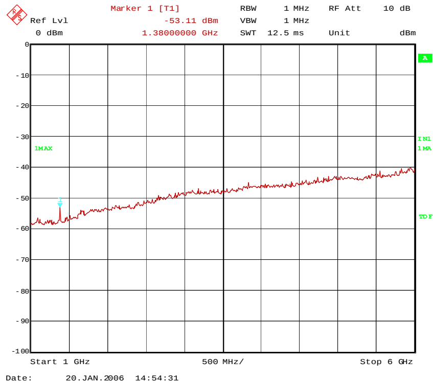
52367_460tx3.wmf: 1 GHz to 6 GHz
