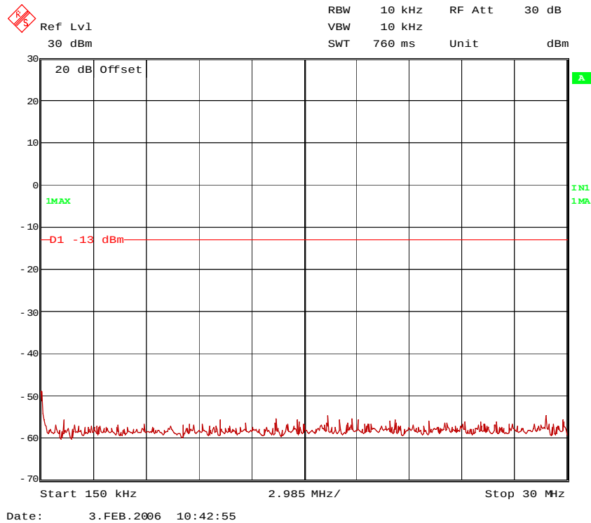
52367c460tx2.wmf: 150 kHz to 30 MHz
