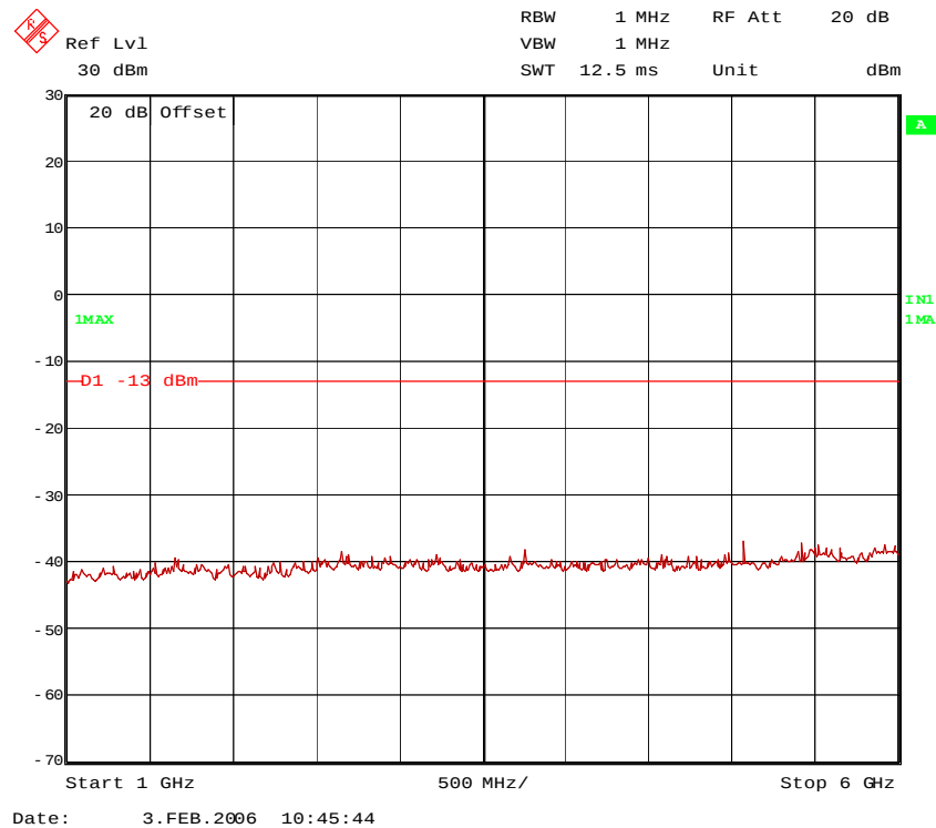
52367c470tx1.wmf: 1 GHz to 6 GHz
