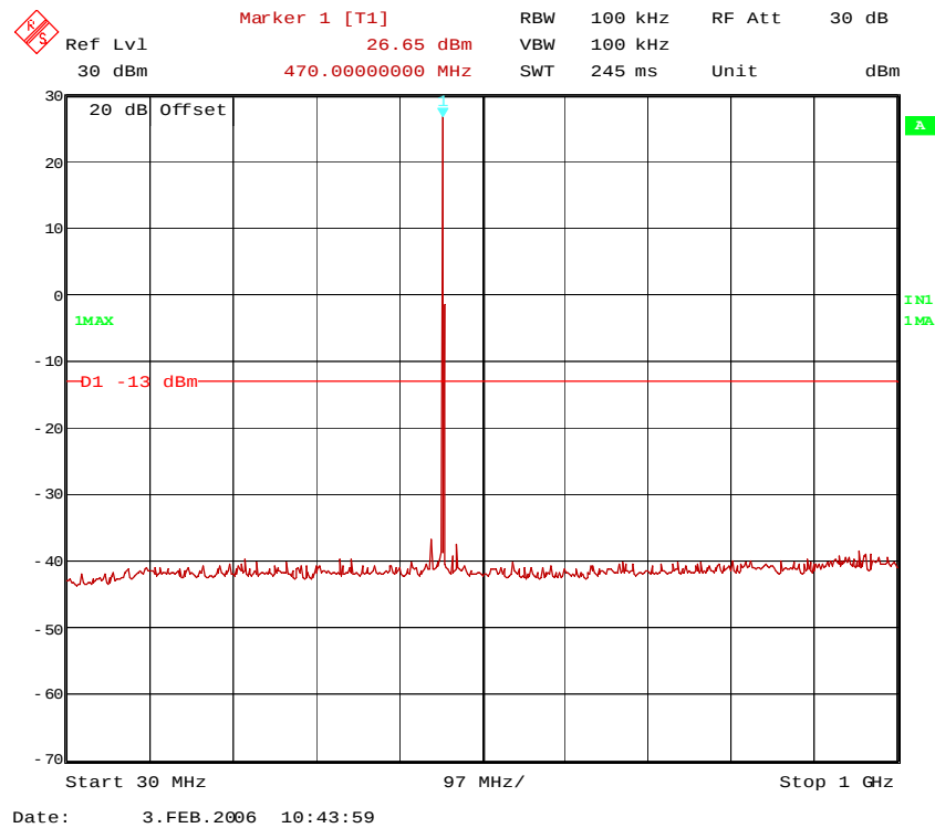
52367c470tx3.wmf: 30 MHz to 1 GHz
