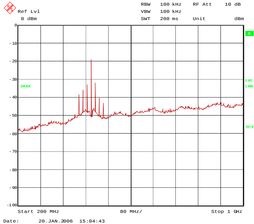
52367_460tx2.wmf: 200 MHz to 1000 MHz
