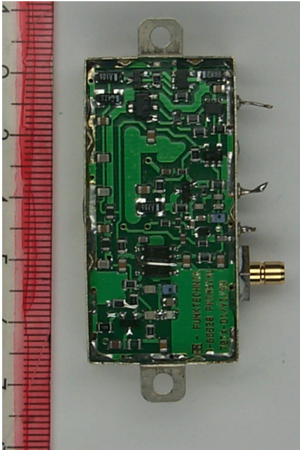
52367_470_4.JPG: PCB, rear view
