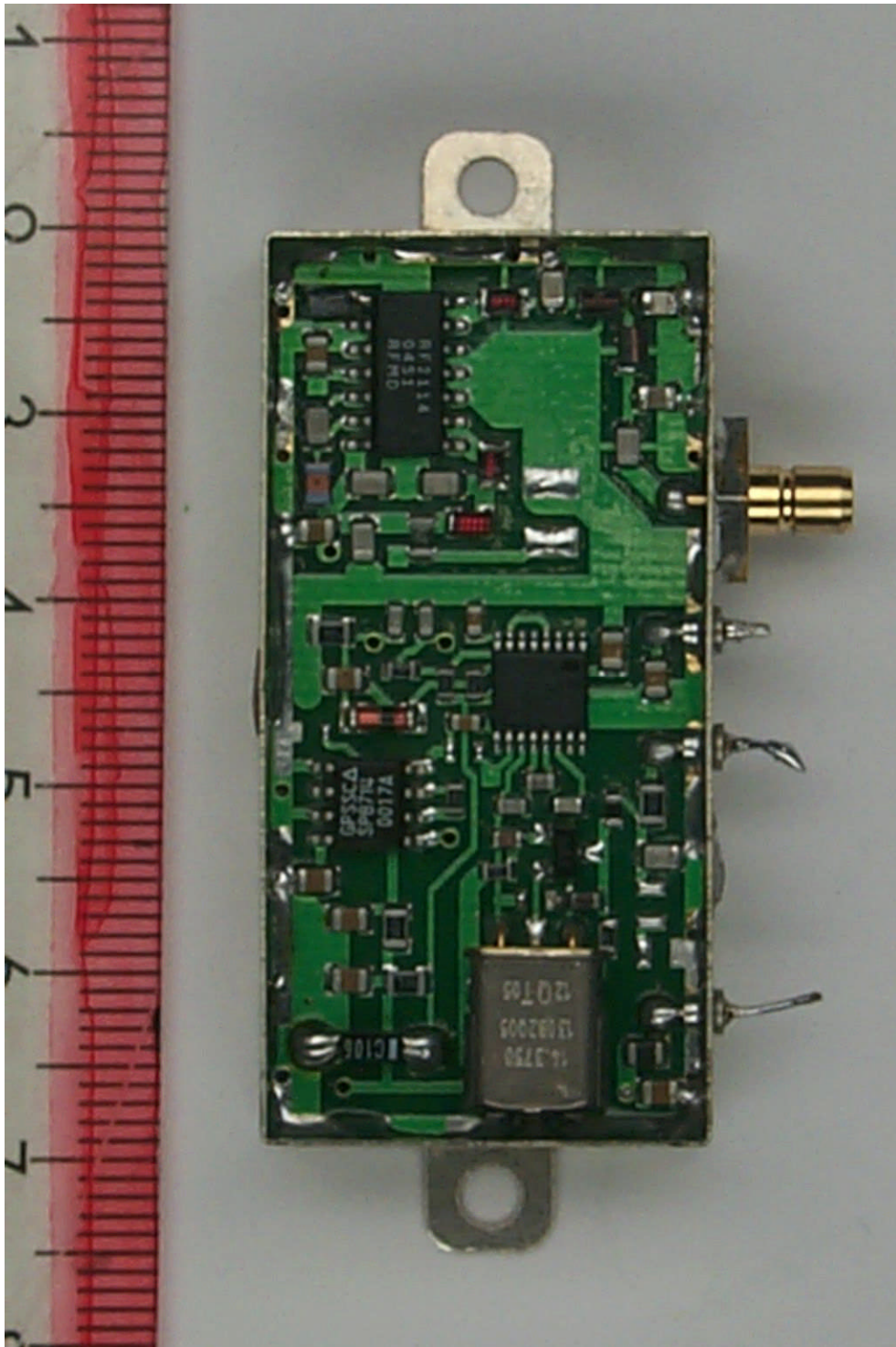
52367_460_2.JPG: PCB, front view
