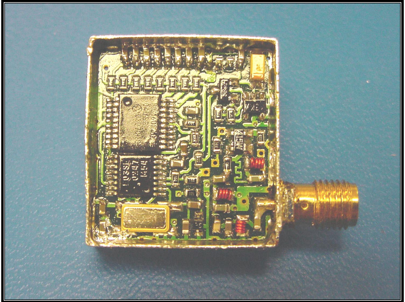
PHOTOGRAPH 13: EUT PCB TOP VIEW
