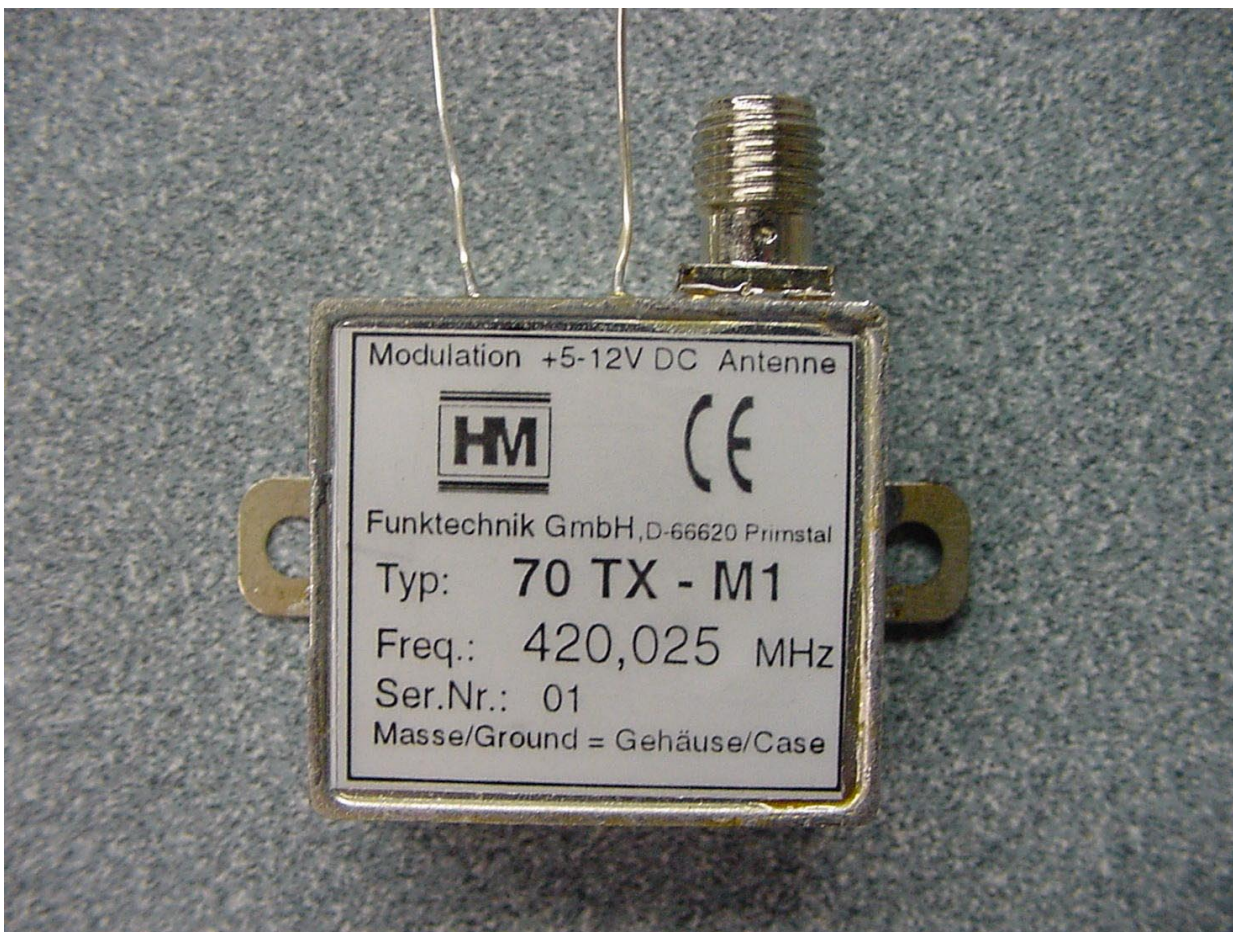
PHOTOGRAPH 5: FRONT VIEW OF TRANSMITTER
