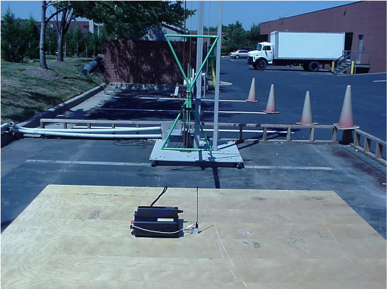
PHOTOGRAPH 1: RADIATED EMISSIONS FRONT VIEW (70 TX-M1)
