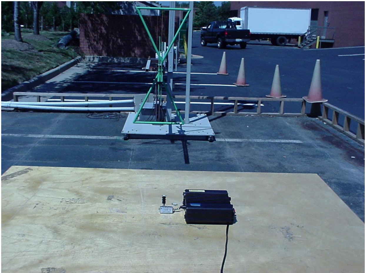
PHOTOGRAPH 3: RADIATED EMISSIONS FRONT VIEW (70 RX-M1)
