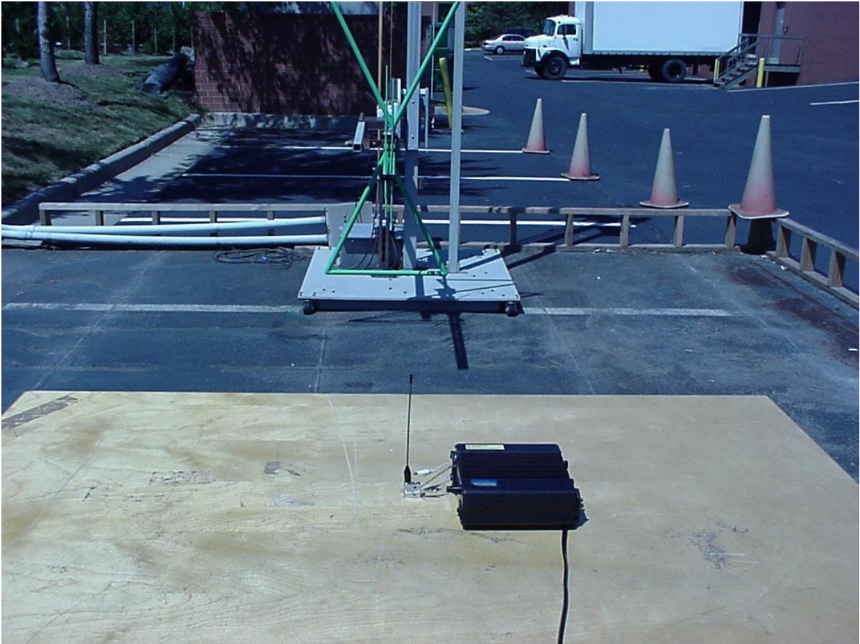
PHOTOGRAPH 2: RADIATED EMISSIONS REAR VIEW (70 TX-M1)
