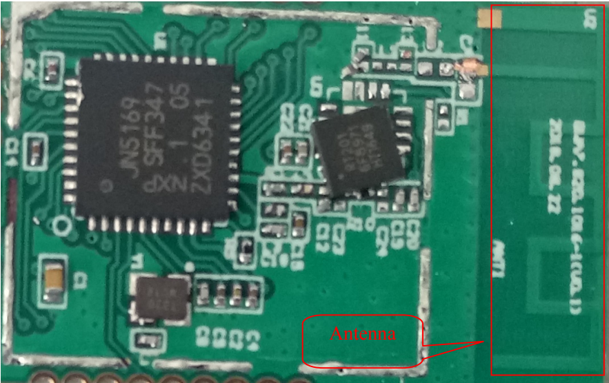
EUT – PCB Top Module View
