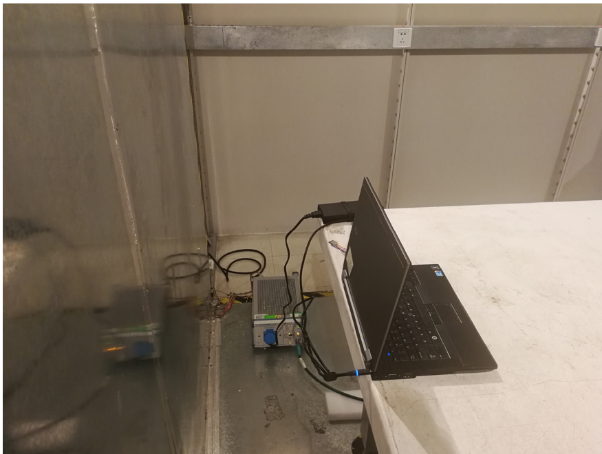
AC Line Conducted Emissions-Rear View
