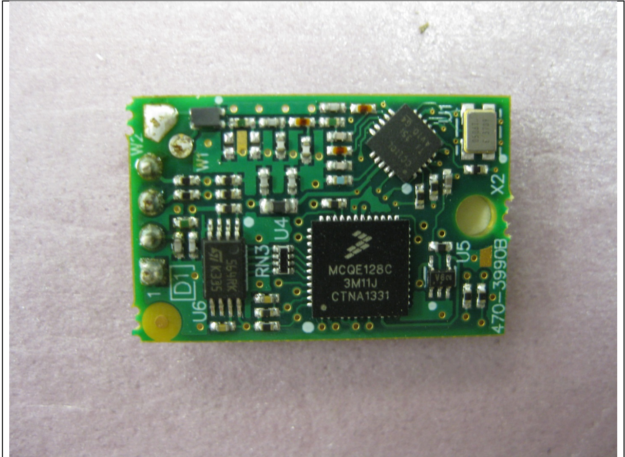
Radio Board – Top
