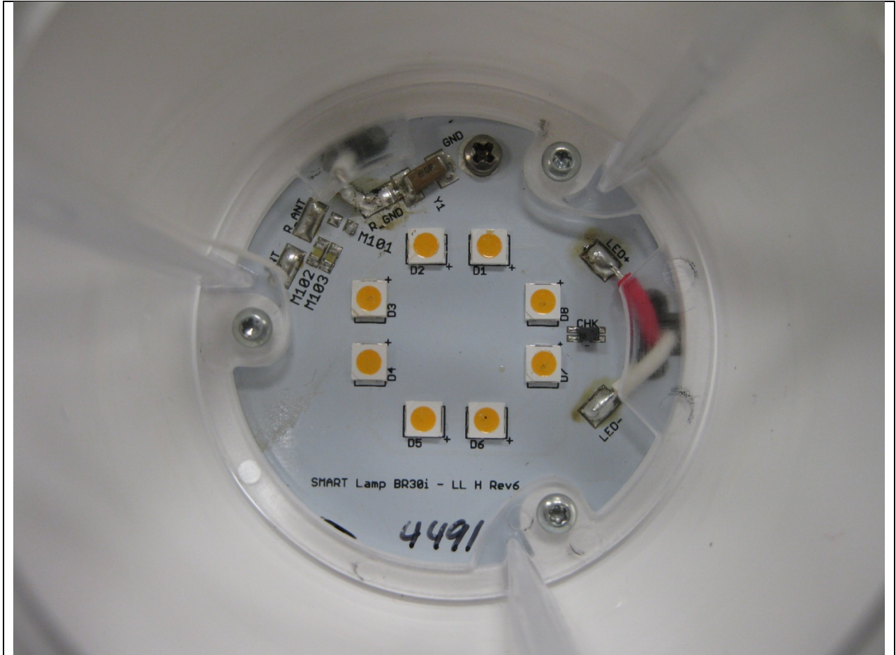
Top of Fixture with Bulb Dome Removed (Zoomed In)
