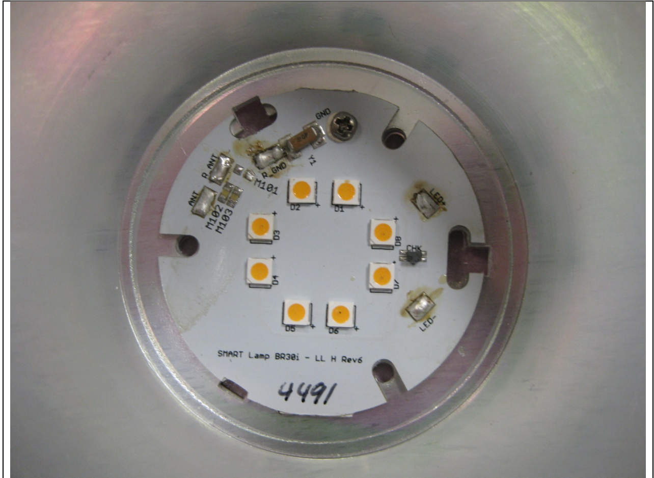
Top of LED Circuit Array – Zoomed In
