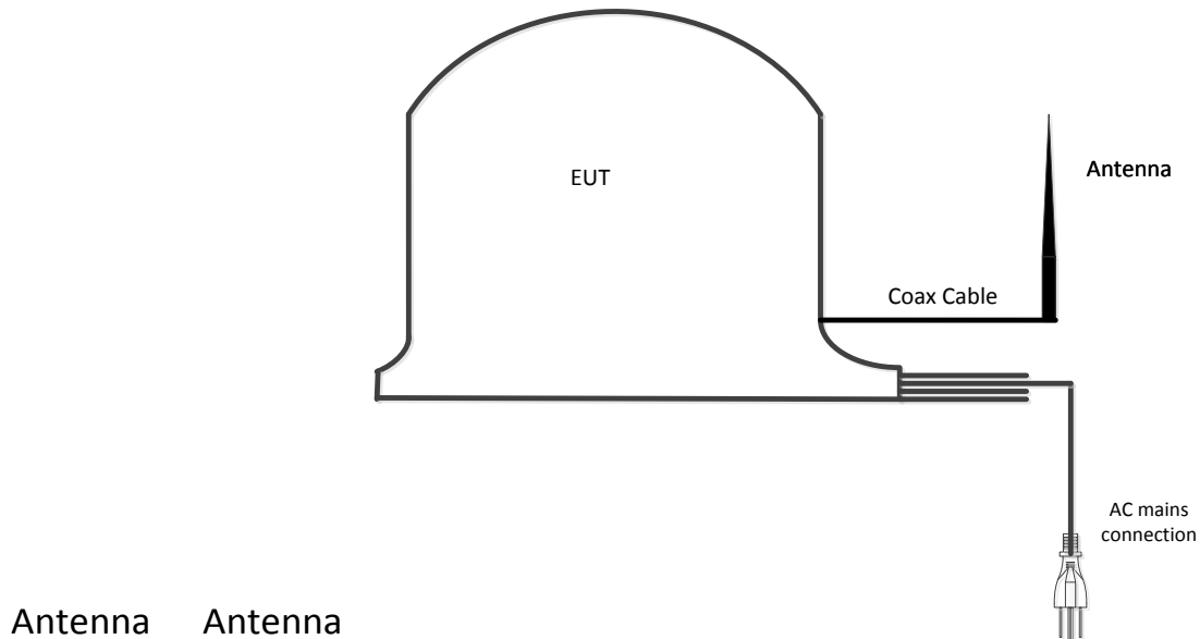
Figure 3.6-1: Setup diagram
