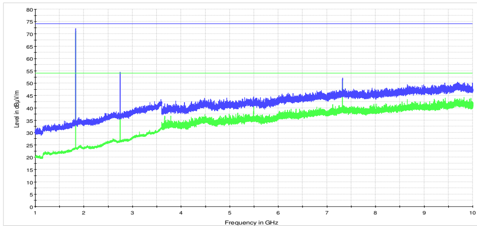
Figure 8.4-7: Radiated spurious emissions for low channel above 1 GHz for restricted band emissions
