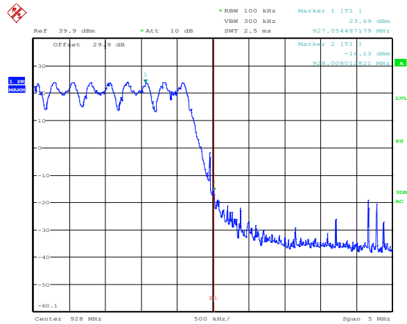
Figure 8.4-11: Upper band edge emission, tx on high channel
