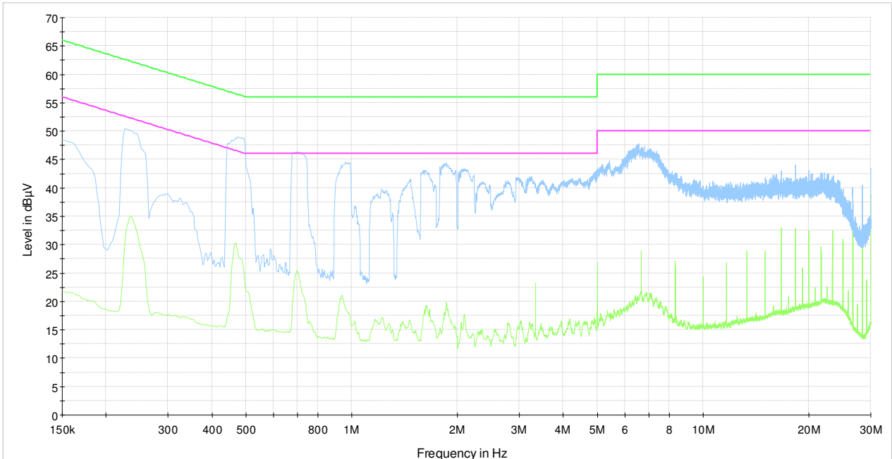
326828_Conducted Emissions_230Vac_Neutral_March 15, 2017
