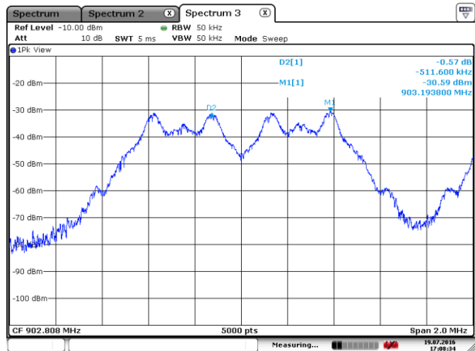
Figure 8.2-4: Carrier frequency separation
