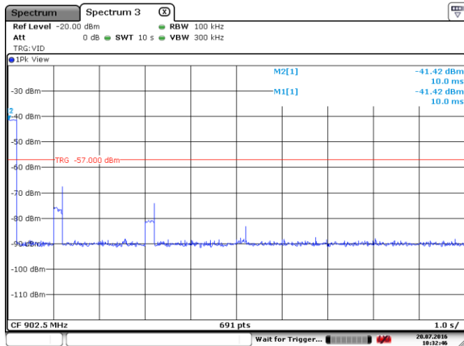
Figure 8.2-6: Number of using of the channel within 10 seconds. Only once.
