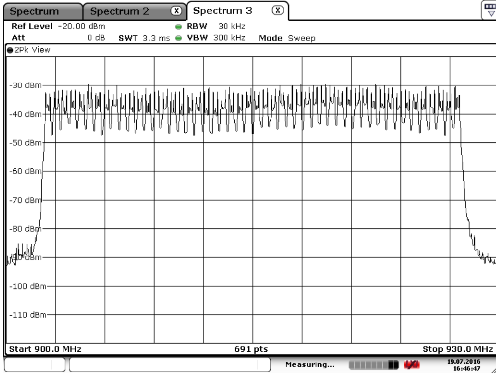
Figure 8.2-5: Number of hopping channels, 50 channels
