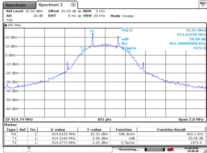
Figure 8.2-2: 20 dB bandwidth on mid channel
