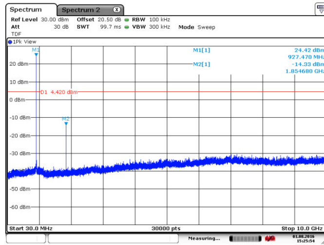
Figure 8.4-3: Conducted spurious emissions for high channel
