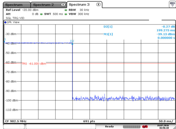
Figure 8.2-7: Dwell time, 199.28 ms
