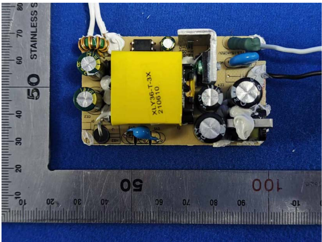
FIGURE 13 CYNCTILE (M/N: CFIXTIHCDEN) POWER BOARD FRONT
