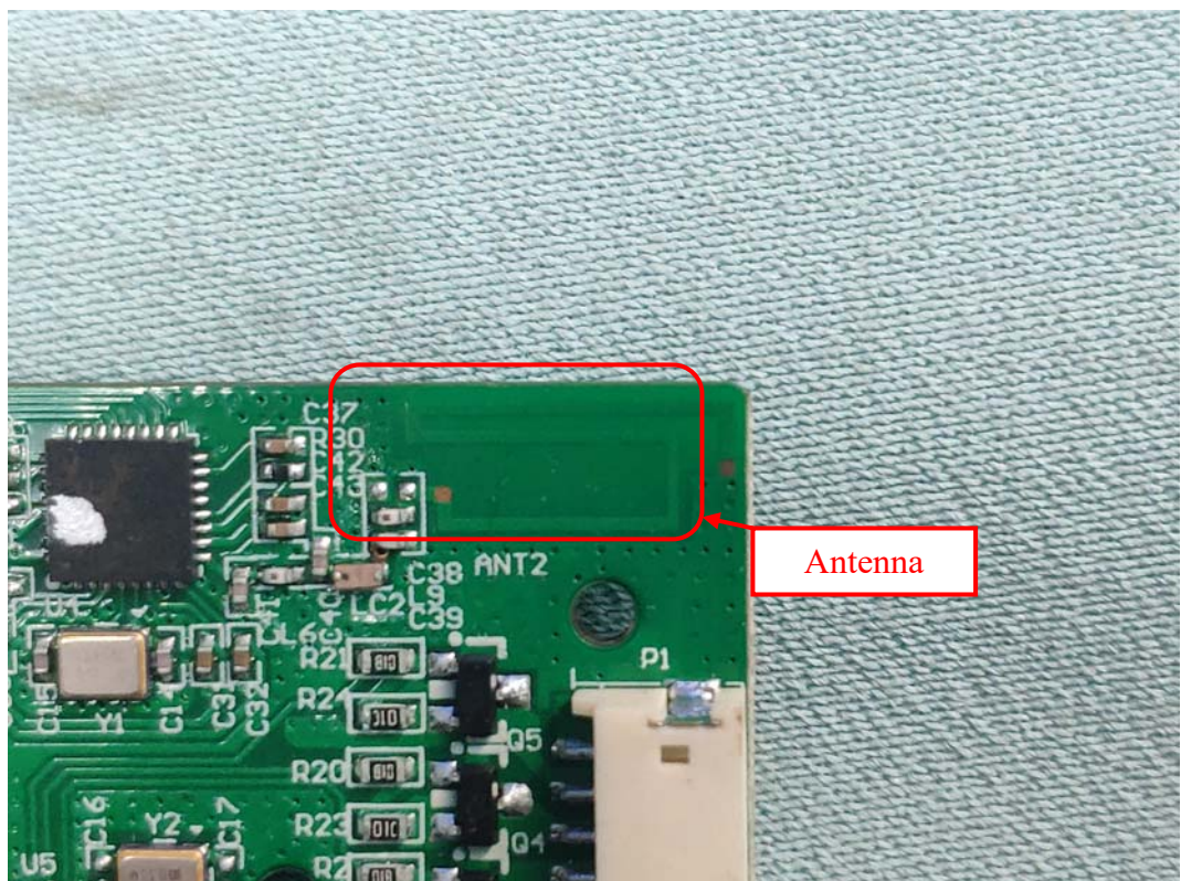
FIGURE 6 CYNC DUAL MODE FULL COLOR LIGHT STRIP (M/N: CLEDSTR20CD1) WLAN ANT (GENERAL VIEW)
