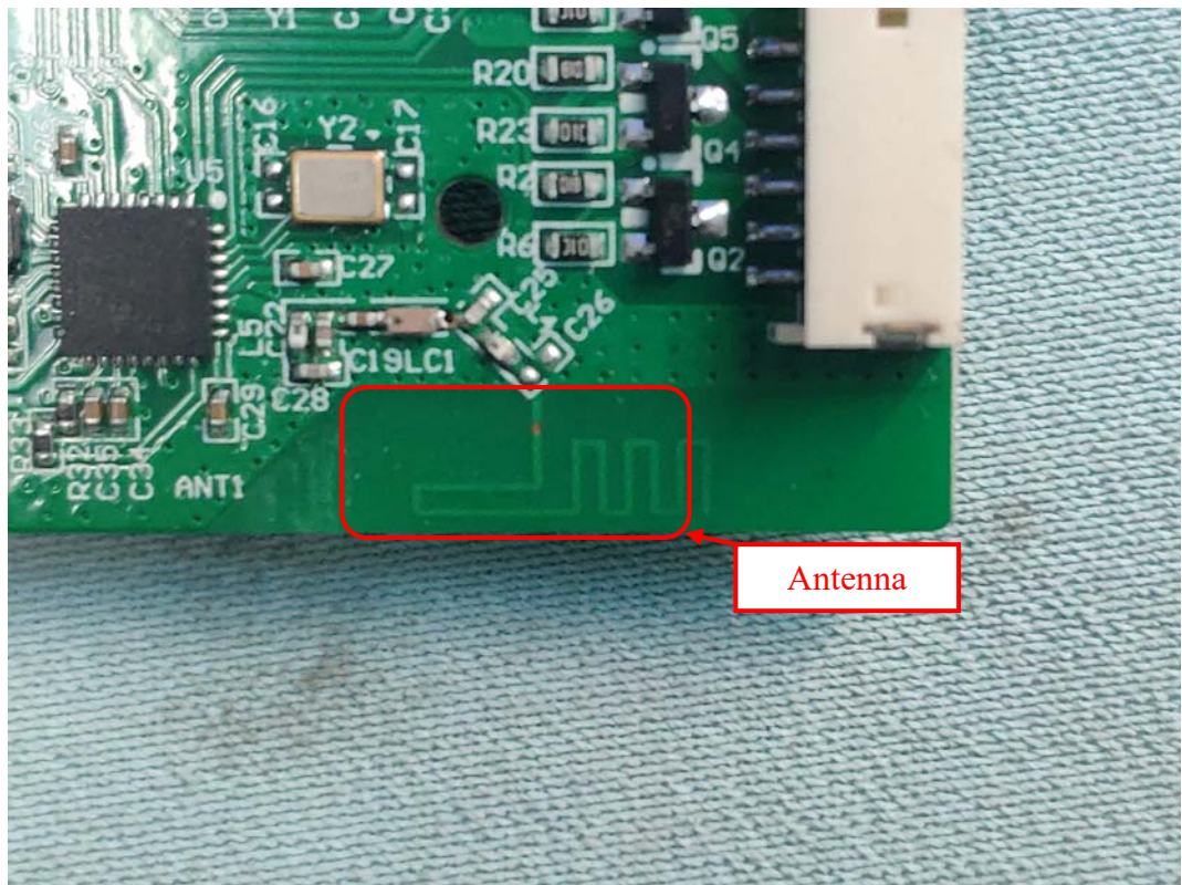
FIGURE 5 CYNC DUAL MODE FULL COLOR LIGHT STRIP (M/N: CLEDSTR20CD1) BLE ANT (GENERAL VIEW)
