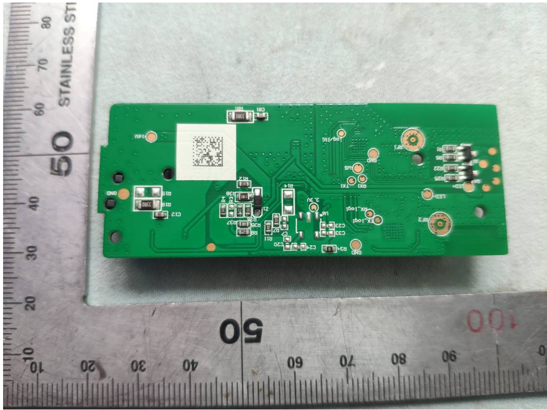
FIGURE 3 CYNCR DUAL MODE FULL COLOR LIGHT STRIP (M/N: CLEDSTR20CD1) MAIN BOARD (SOLDERED SIDE)
