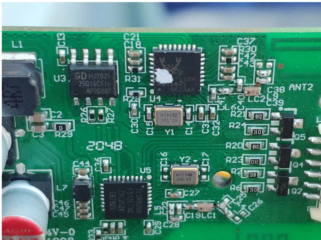
FIGURE 4 CYNCR DUAL MODE FULL COLOR LIGHT STRIP (M/N: CLEDSTR20CD1) CHIP&CRYSTAL MAIN BOARD (COMPONENT SIDE)
