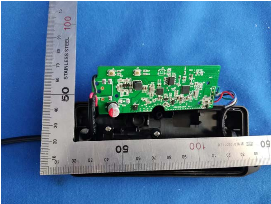
FIGURE 4 CYNCR DIRECT CONNECTED OUTDOOR PREMIUM LIGHT STRIP (32FT.) (M/N: CLEDSTR36LCDODP) CHIP & CRYSTAL ON RBOARD
