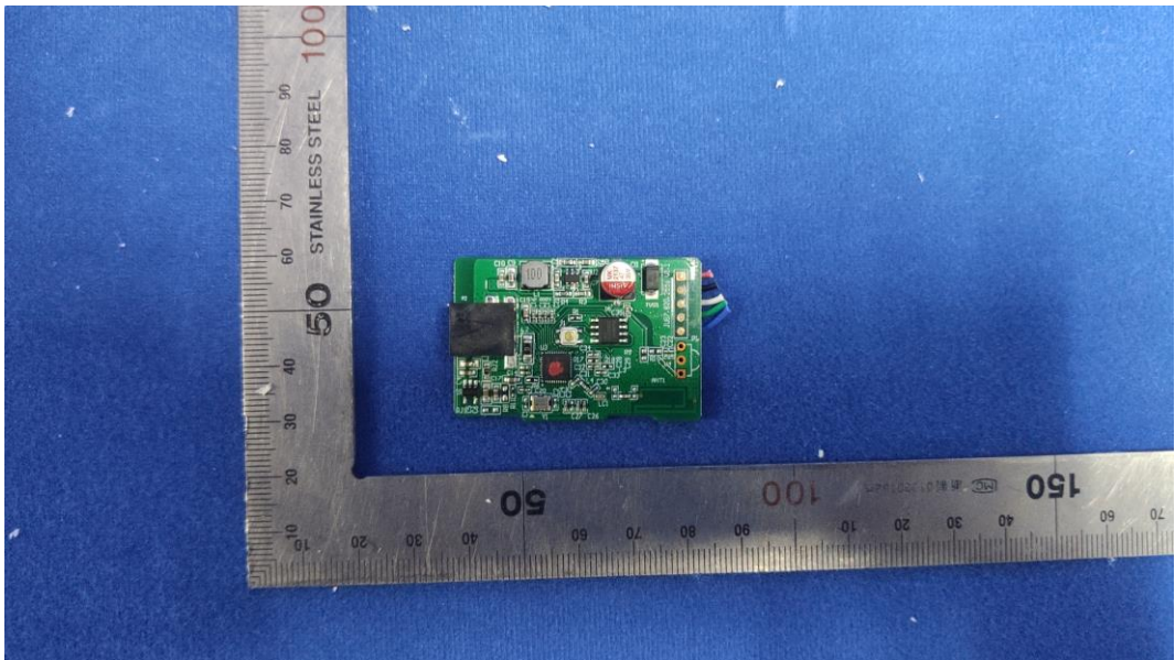
FIGURE 6 CYNC DIRECT CONNECTED INDOOR LIGHT STRIP (16FT.) (M/N: CLEDSTR12CDIDB) CONTROLBOARD BACK
