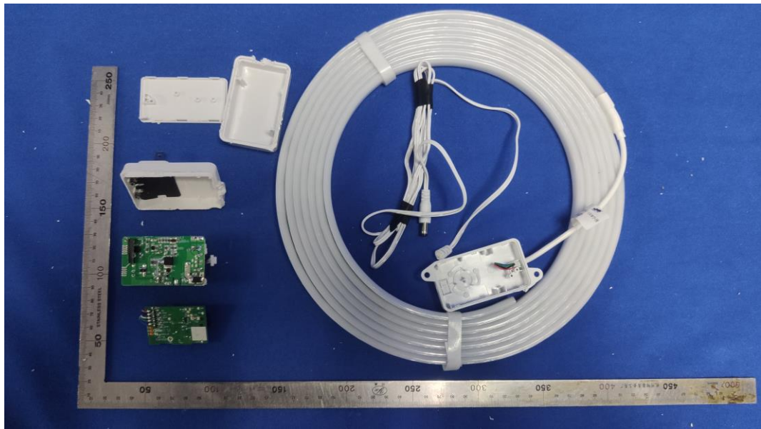
FIGURE 2 CYNC DIRECT CONNECTED INDOOR LIGHT STRIP (16FT.) (M/N: CLEDSTR12CDIDB) COVER REMOVED #1
