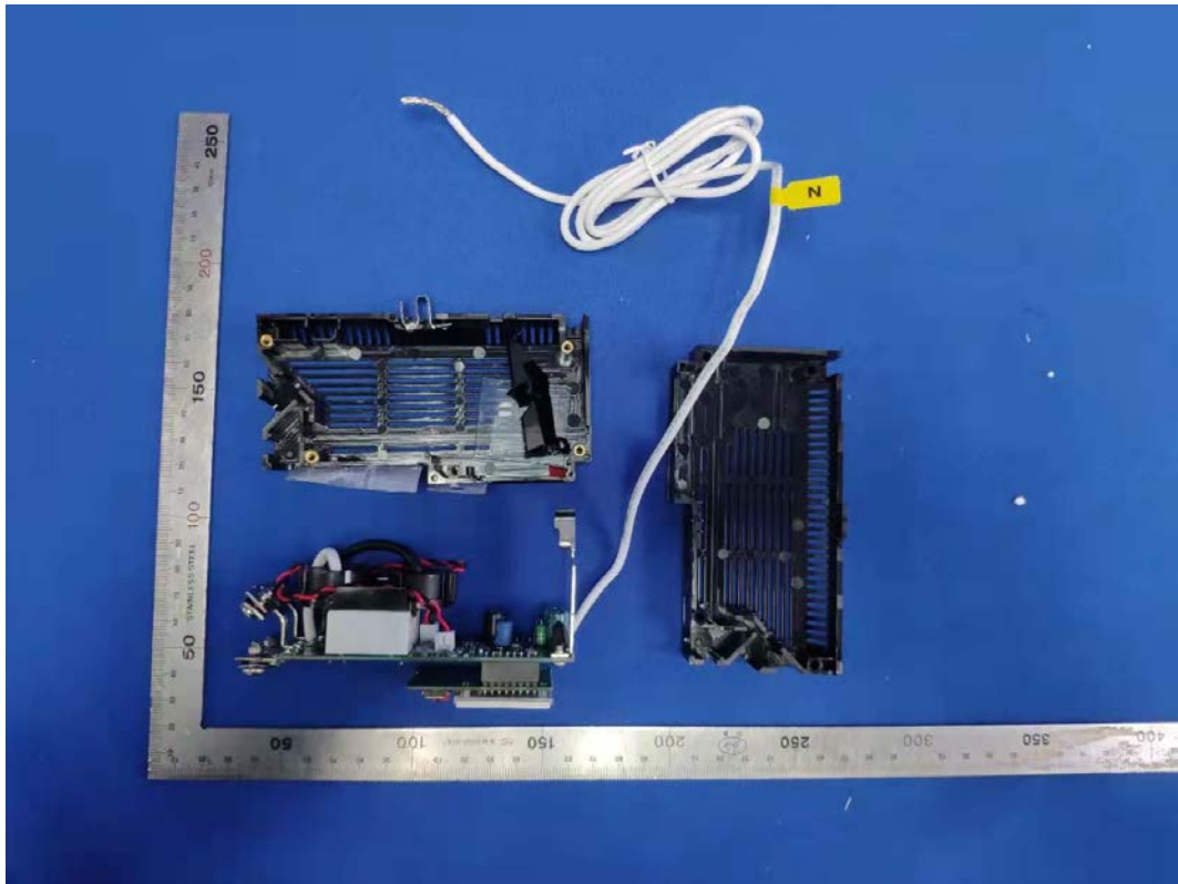
FIGURE 1 QO DUAL 20A RELAY, WITH CT, PIGTAIL (M/N: GPM-Q2R20120-21) COVER REMOVE
