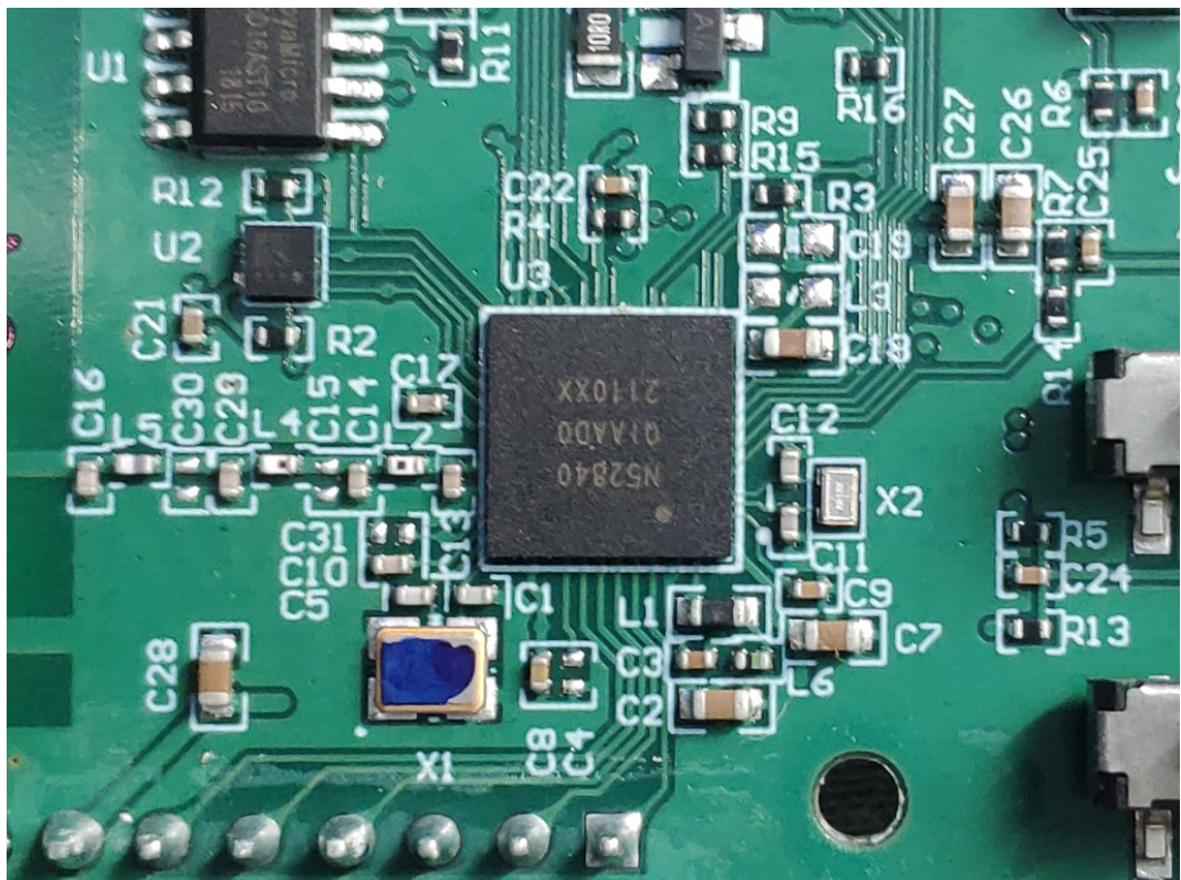
FIGURE 7 QO DUAL 20A RELAY, WITH CT, PIGTAIL (M/N: GPM-Q2R20120-21) CHIP & CRYSTAL ON RBOARD
