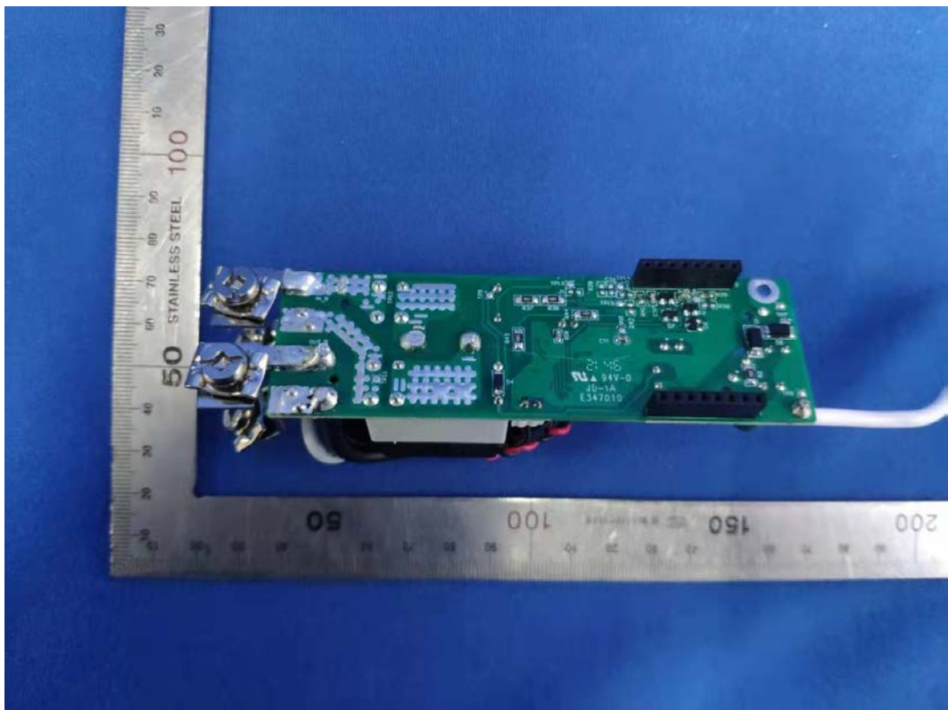
FIGURE 3 QO DUAL 20A RELAY, WITH CT, PIGTAIL (M/N: GPM-Q2R20120-21) MAINBOARD BACK
