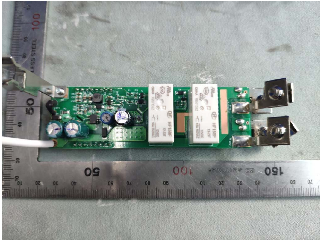
FIGURE 10 QO DUAL 24V CONTROL RELAY, PON (M/N: GPM-QP2PWL-21) MAINBOARD BACK VIEW
