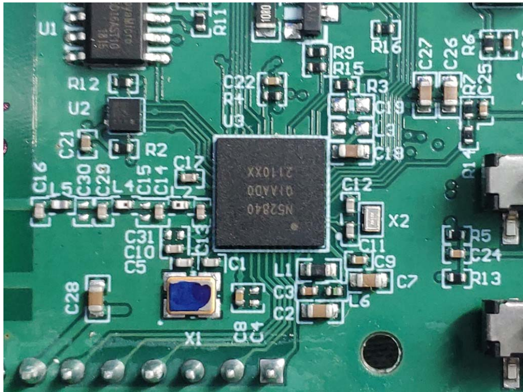
FIGURE 13 QO DUAL 24V CONTROL RELAY, PON (M/N: GPM-QP2PWL-21) CHIP AND CRYSTAL ON RF BOARD
