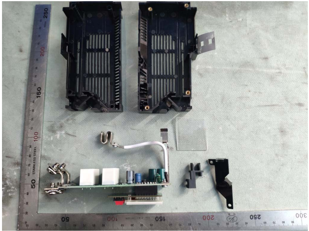
FIGURE 8 QO DUAL 24V CONTROL RELAY, PON (M/N: GPM-QP2PWL-21) COVER REMOVED
