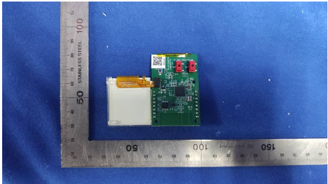
FIGURE 12 QO DUAL 24V CONTROL RELAY, PON (M/N: GPM-QP2PWL-21) RF BOARD BACK VIEW
