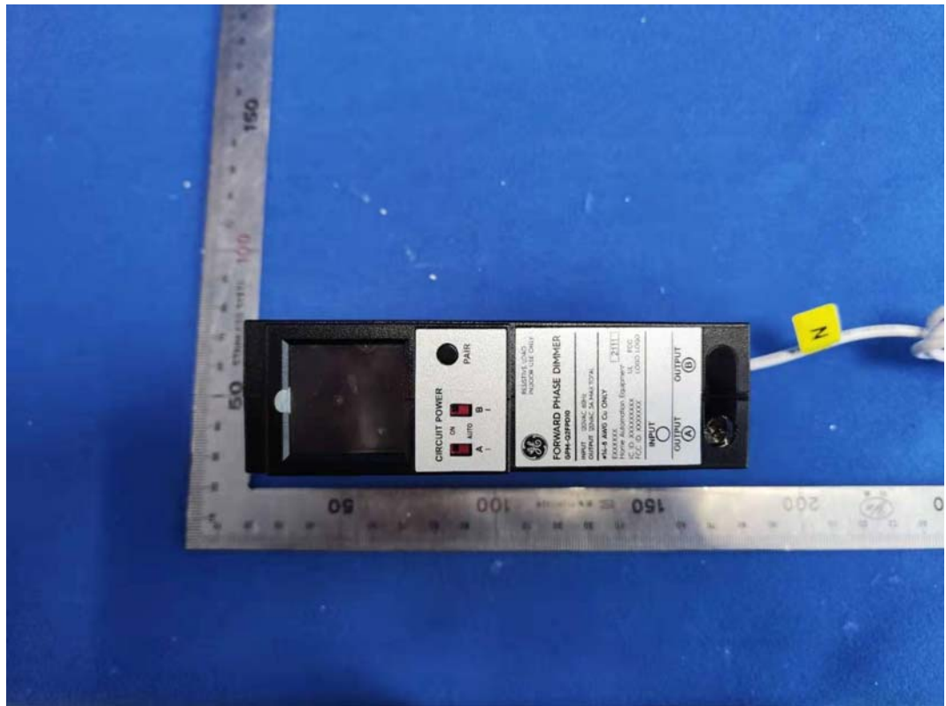
FIGURE 6 QO FORWARD PHASE DIMMER, PIGTAIL (M/N: GPM-Q2FPD05-21) RIGHT
