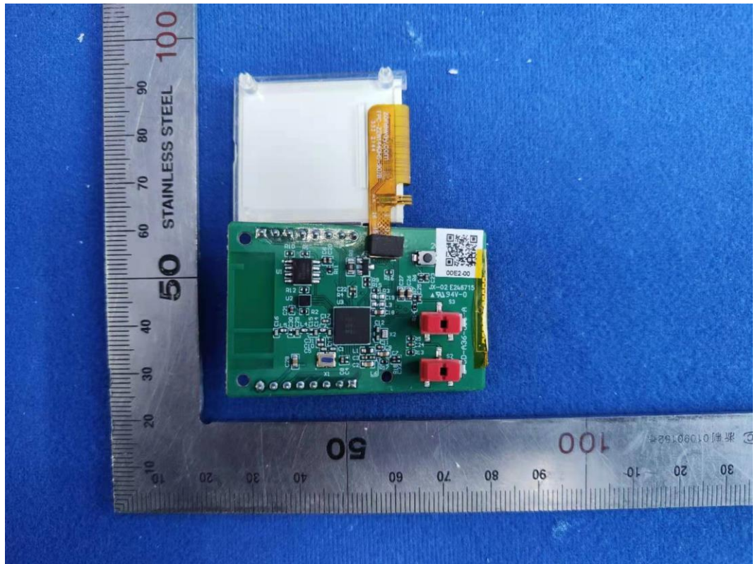
FIGURE 14 QO ADAPTIVE PHASE DIMMER, PIGTAIL (M/N: GPM-Q2APD10-21) RF BOARD BACK
