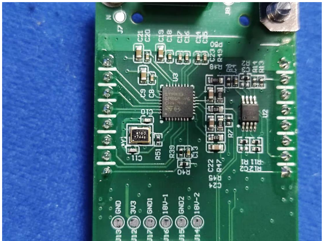
FIGURE 10 QO ADAPTIVE PHASE DIMMER, PIGTAIL (M/N: GPM-Q2APD10-21) CHIP & CRYSTAL ON POWERBOARD
