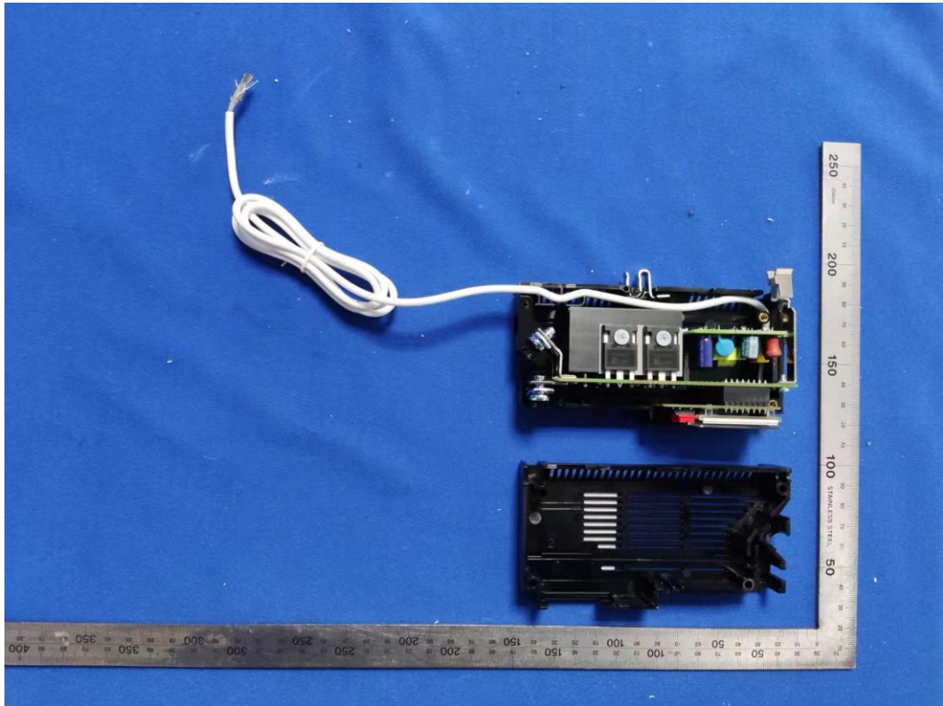
FIGURE 8 QO ADAPTIVE PHASE DIMMER, PIGTAIL (M/N: GPM-Q2APD10-21) POWERBOARD FRONT
