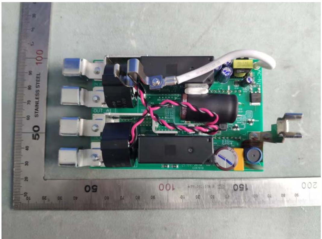
FIGURE 8 QO 60A RELAY WITH CURRENT TRANSFORMER PON (M/N: GPM-QP1R60240-21) MAINBOARD FRONT
