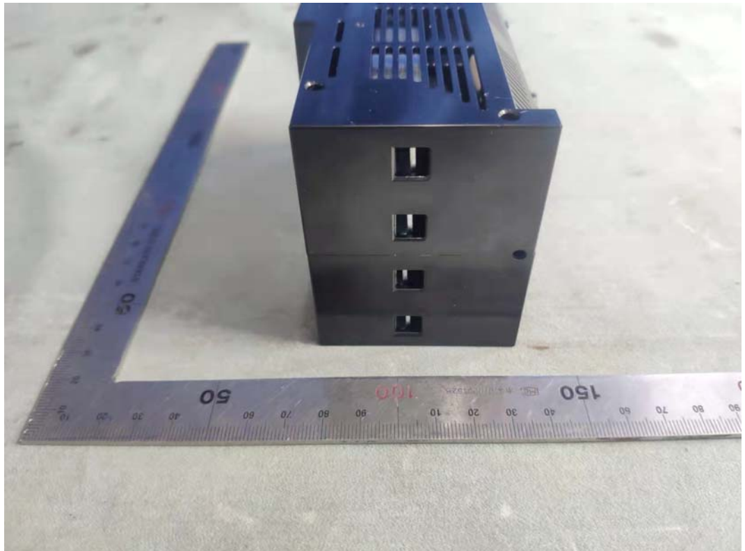
FIGURE 2 QO 60A RELAY WITH CURRENT TRANSFORMER PON (M/N: GPM-QP1R60240-21) BACK
