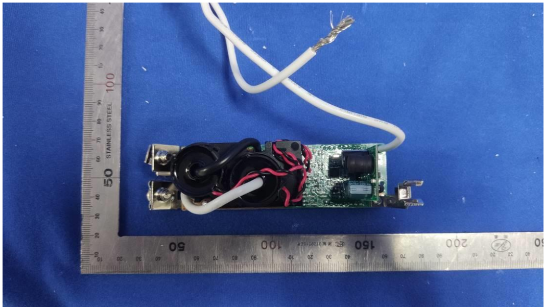
FIGURE 15 QO 240V 2-POLE RELAY, WITH CT, PIGTAIL (M/N: GPM-Q1R30240-21) MAINBOARD BACK
