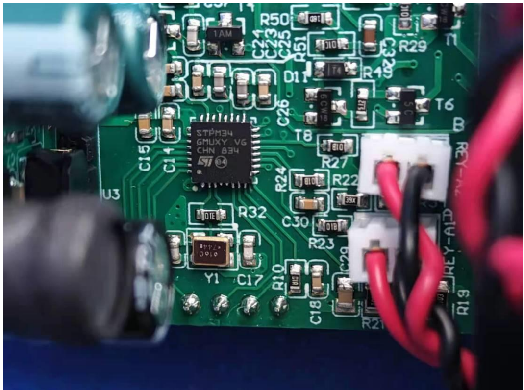
FIGURE 16 QO 240V 2-POLE RELAY, WITH CT, PIGTAIL (M/N: GPM-Q1R30240-21) CHIP & CRYSTAL ON BOARD
