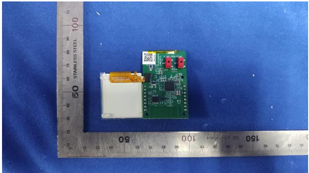
FIGURE 17 QO 240V 2-POLE RELAY, WITH CT, PIGTAIL (M/N: GPM-Q1R30240-21) RF BOARD FRONT
