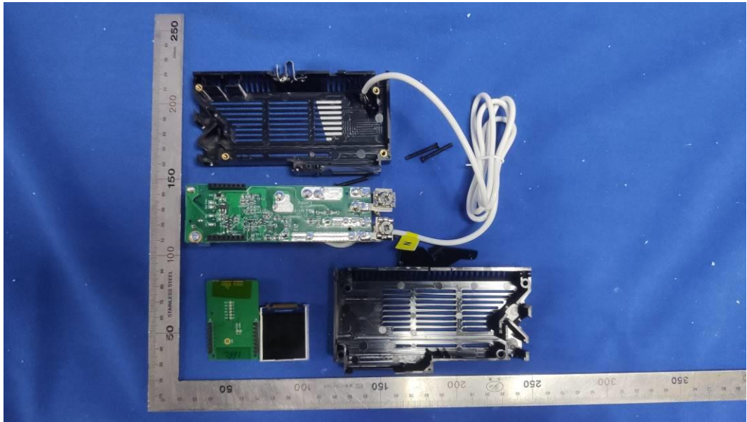
FIGURE 13 QO 240V 2-POLE RELAY, WITH CT, PIGTAIL (M/N: GPM-Q1R30240-21) COVER REMOVE
