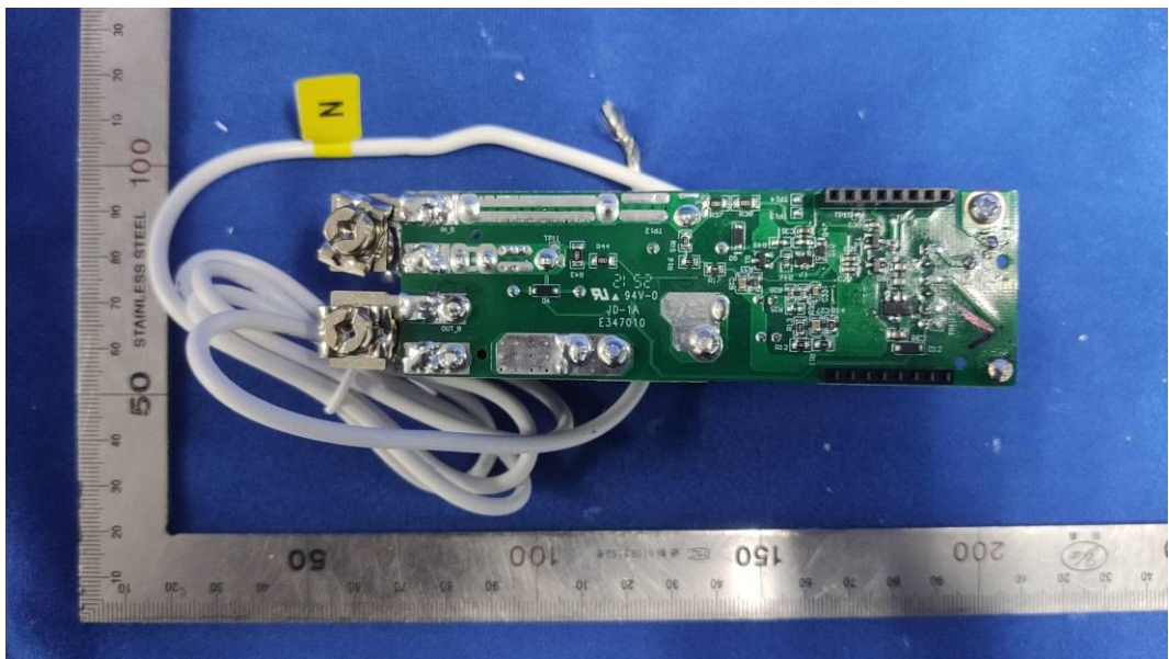
FIGURE 14 QO 240V 2-POLE RELAY, WITH CT, PIGTAIL (M/N: GPM-Q1R30240-21) MAINBOARD FRONT
