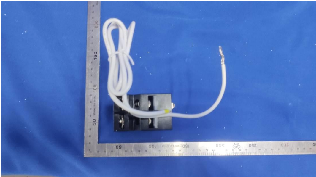
FIGURE 10 QO 240V 2-POLE RELAY, WITH CT, PIGTAIL (M/N: GPM-Q1R30240-21) RIGHT
