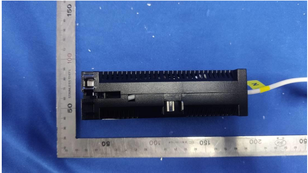
FIGURE 9 QO 240V 2-POLE RELAY, WITH CT, PIGTAIL (M/N: GPM-Q1R30240-21) BACK
