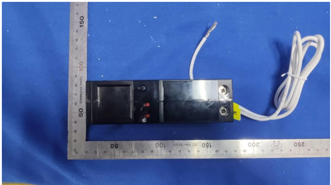
FIGURE 8 QO 240V 2-POLE RELAY, WITH CT, PIGTAIL (M/N: GPM-Q1R30240-21) FRONT
