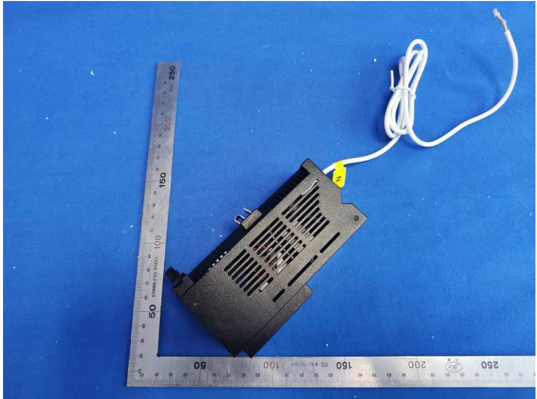
FIGURE 7 QO 240V 2-POLE RELAY, WITH CT, PIGTAIL (M/N: GPM-Q1R30240-21) GENERAL
