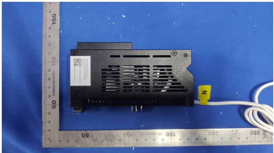
FIGURE 12 QO 240V 2-POLE RELAY, WITH CT, PIGTAIL (M/N: GPM-Q1R30240-21) BOTTOM
