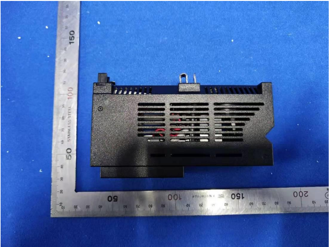
FIGURE 6 QO 240V 2-POLE RELAY, WITH CT, PON (M/N: GPM-QP1R30240-21) BOTTOM
