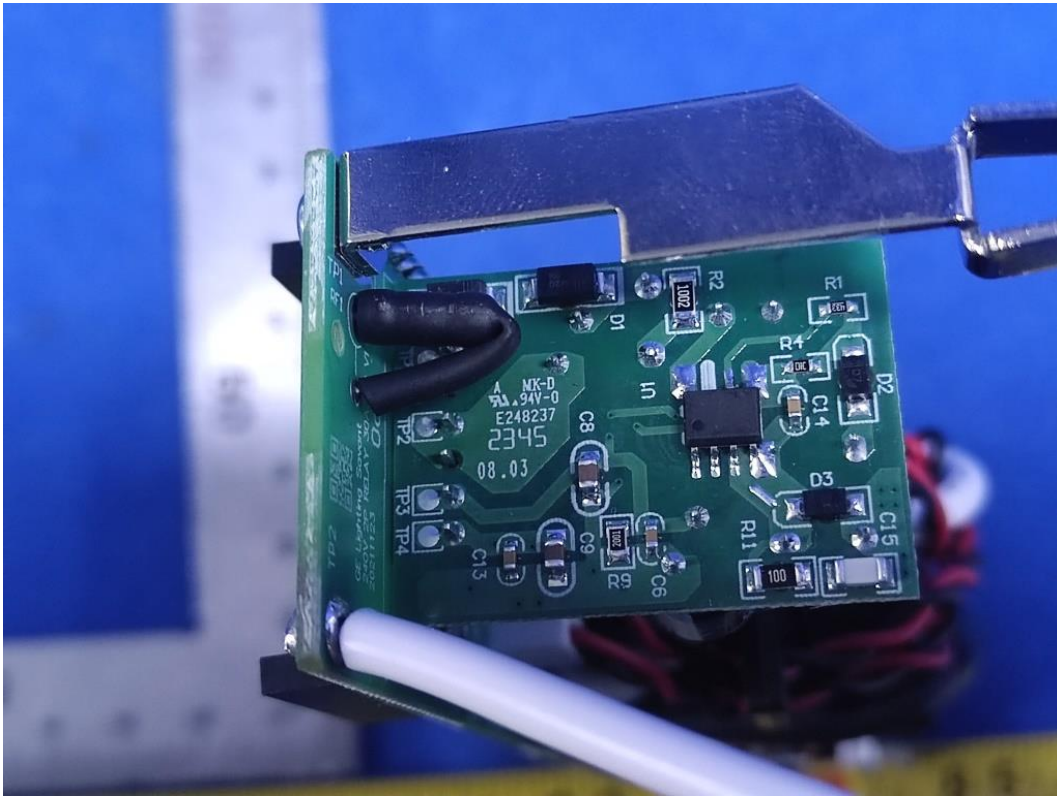
FIGURE 11 240 VAC 30 A WISER CONTROL RELAY (QO200PWX240) MAINBOARD FRONT
