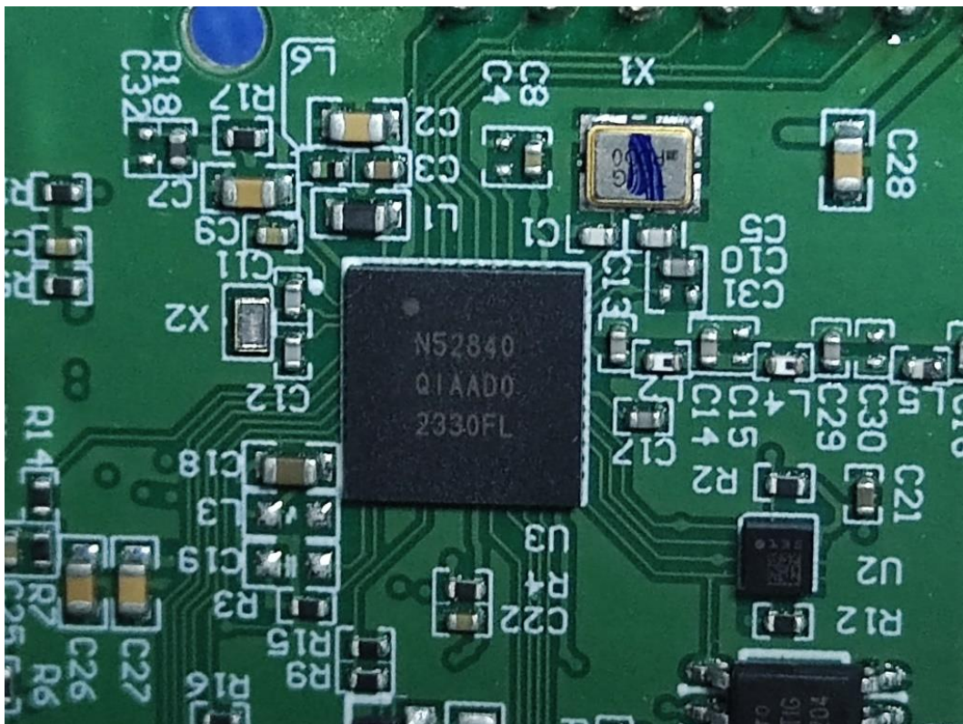
FIGURE 16 240 VAC 30 A WISER CONTROL RELAY (QO200PWX240) CHIP&CRYSTAL ON RF BOARD
