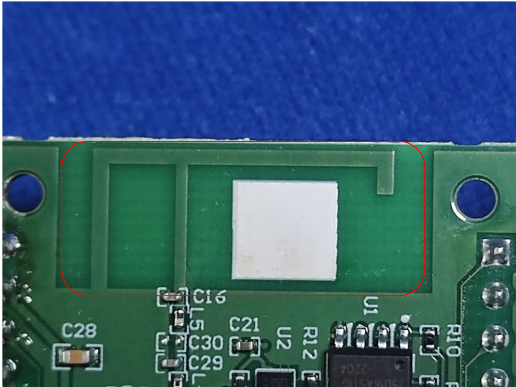
FIGURE 17 240 VAC 30 A WISER CONTROL RELAY (QO200PWX240) ANTENNA
