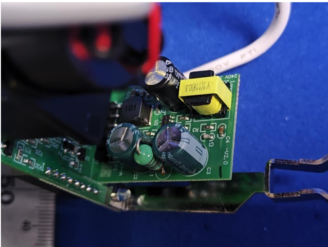
FIGURE 12 240 VAC 30 A WISER CONTROL RELAY (QO200PWX240) MAINBOARD BACK
