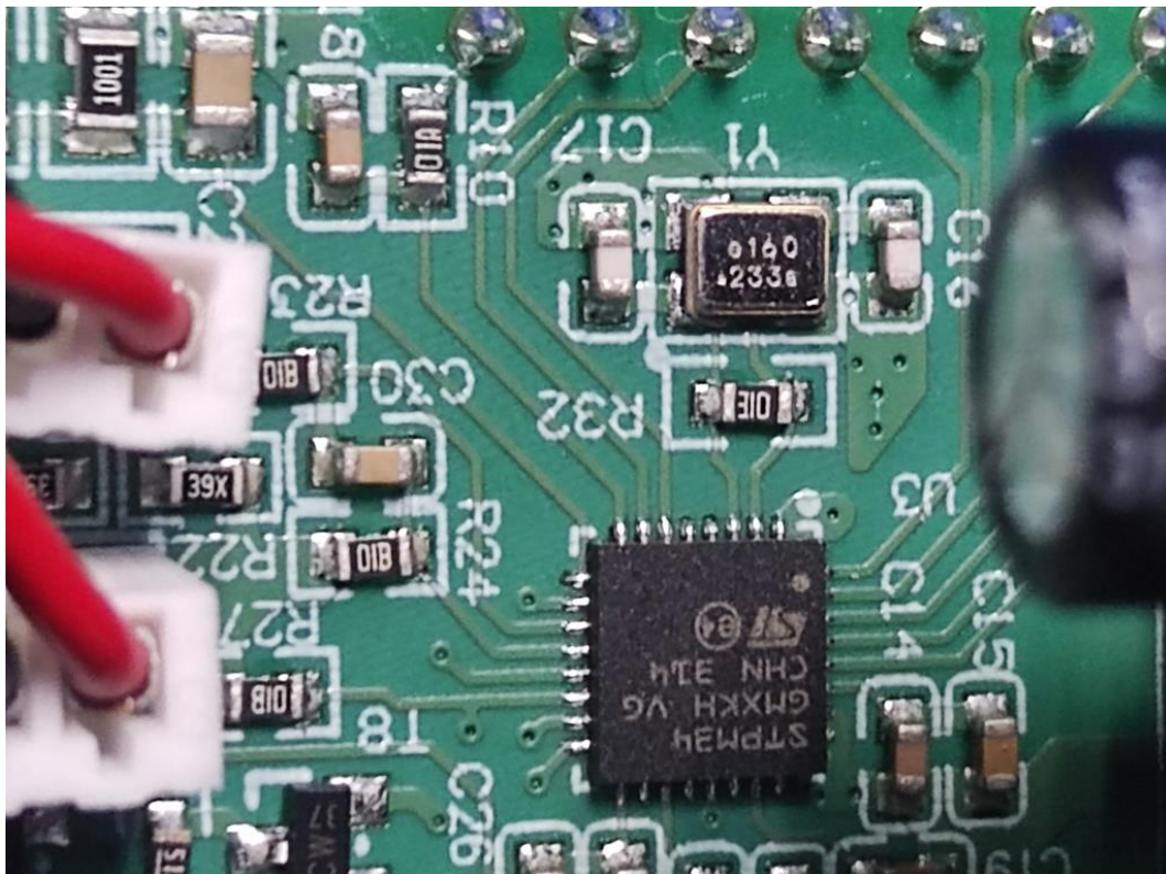
FIGURE 10 240 VAC 30 A WISER CONTROL RELAY (QO200PWX240) CHIP & CRYSTAL ON POWER BOARD
