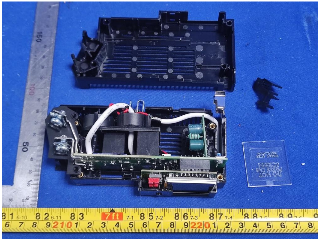
FIGURE 8 240 VAC 30 A WISER CONTROL RELAY (QO200PWX240) POWER BOARD FRONT
