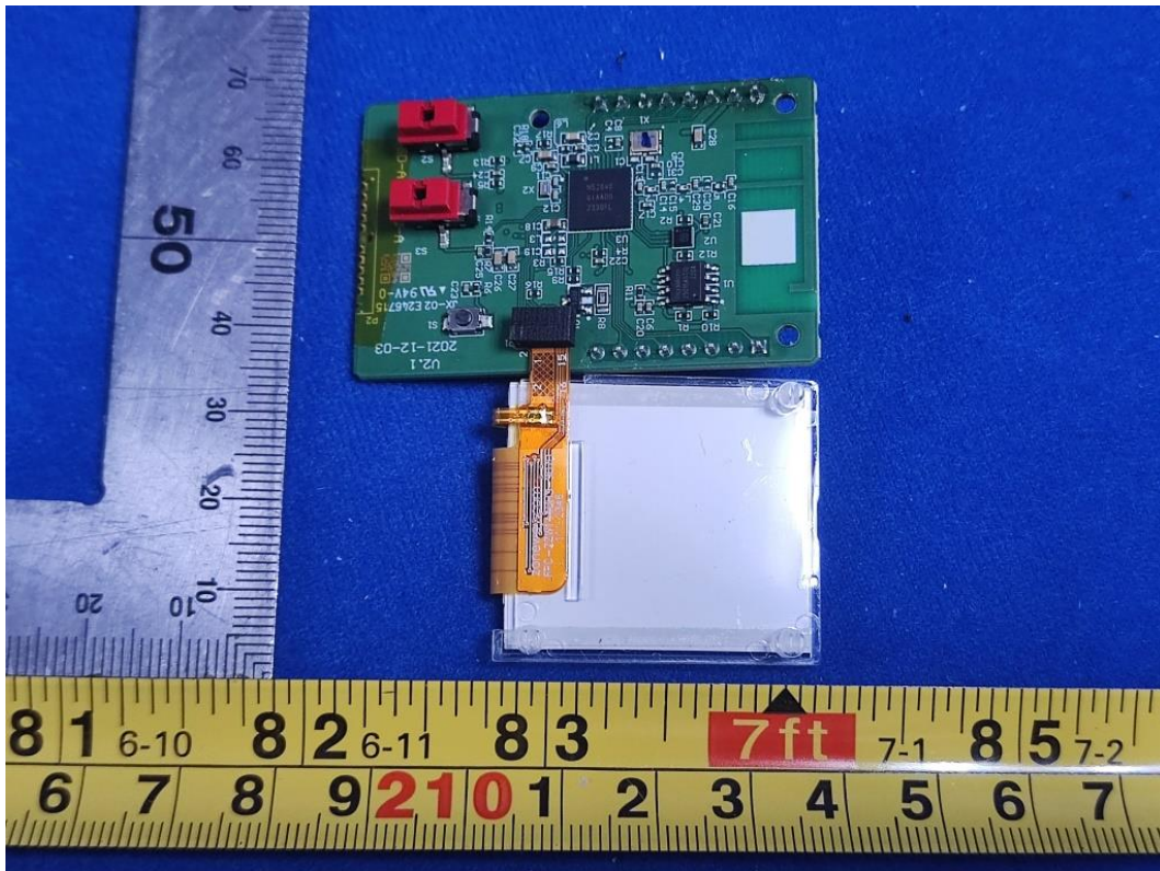
FIGURE 15 240 VAC 30 A WISER CONTROL RELAY (QO200PWX240) RF BOARD VIEW
