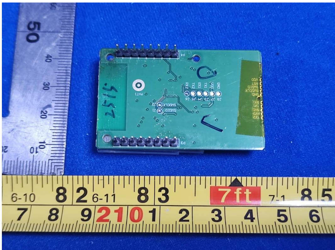
FIGURE 14 240 VAC 30 A WISER CONTROL RELAY (QO200PWX240) RF BOARD BACK
