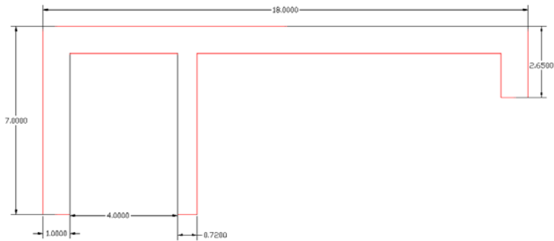
Antenna picture (unit: mm)
