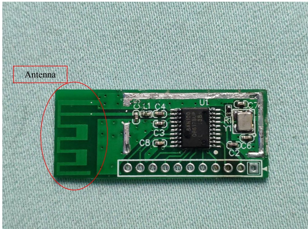
FIGURE 3 GE LINKABLE 2.4G MODEL (M/N: OBM1000CTSD01) CHIP & CRYSTAL ON MAIN BOARD
