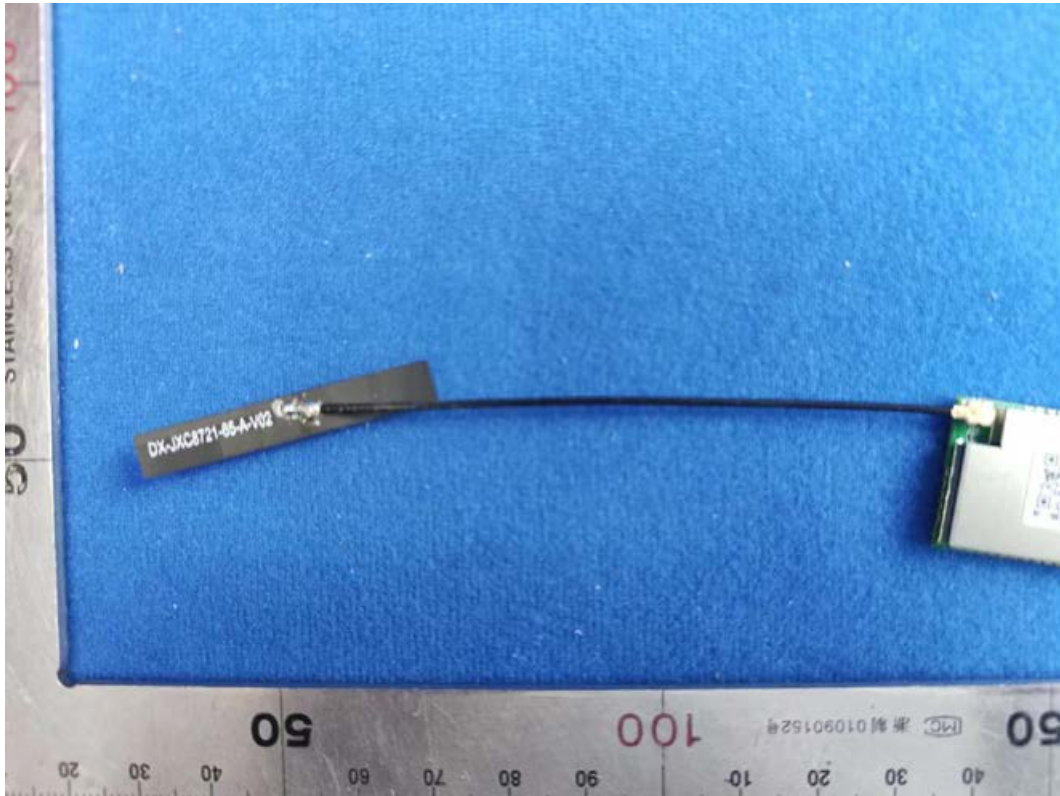
FIGURE 5 RTL8721DM MODULE (M/N: JXC8721-65) ANTENNA
