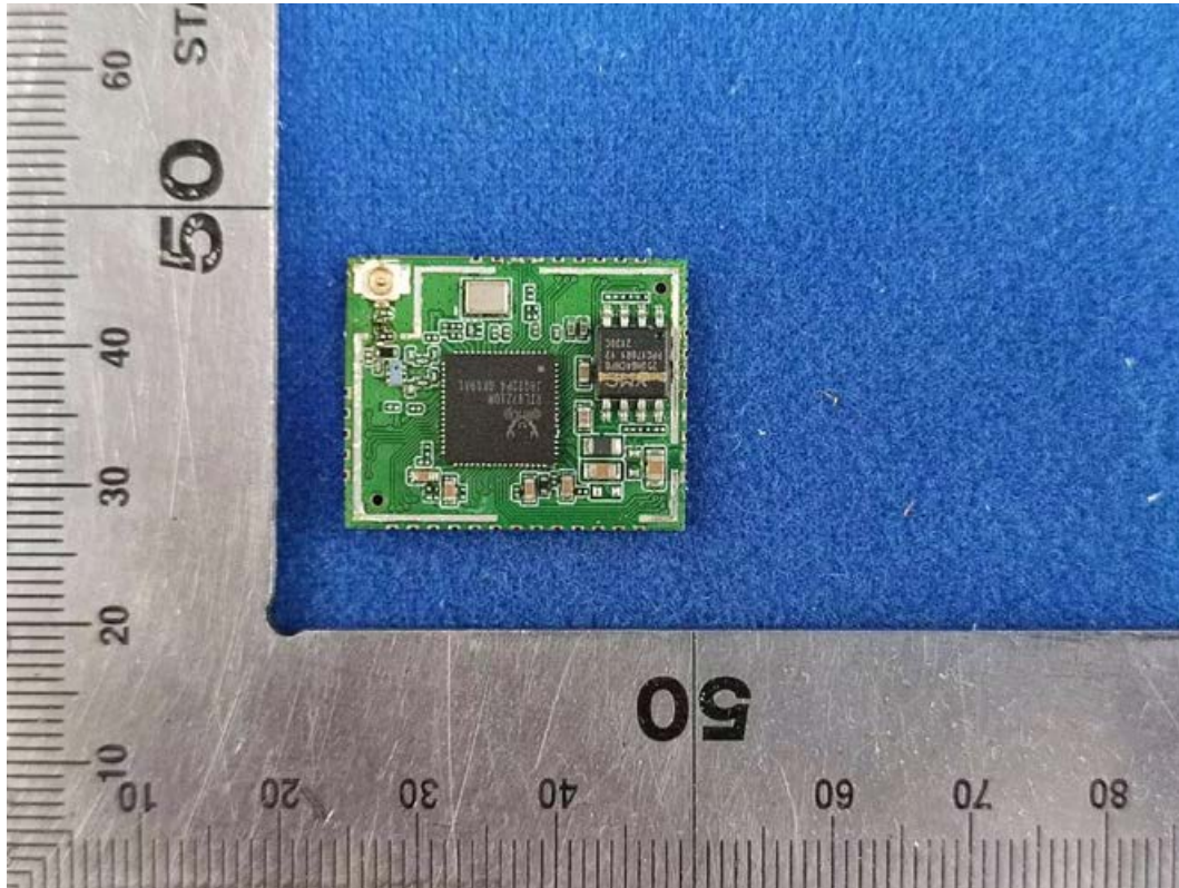
FIGURE 4 RTL8721DM MODULE (M/N: JXC8721-65) CHIP & CRYSTAL
