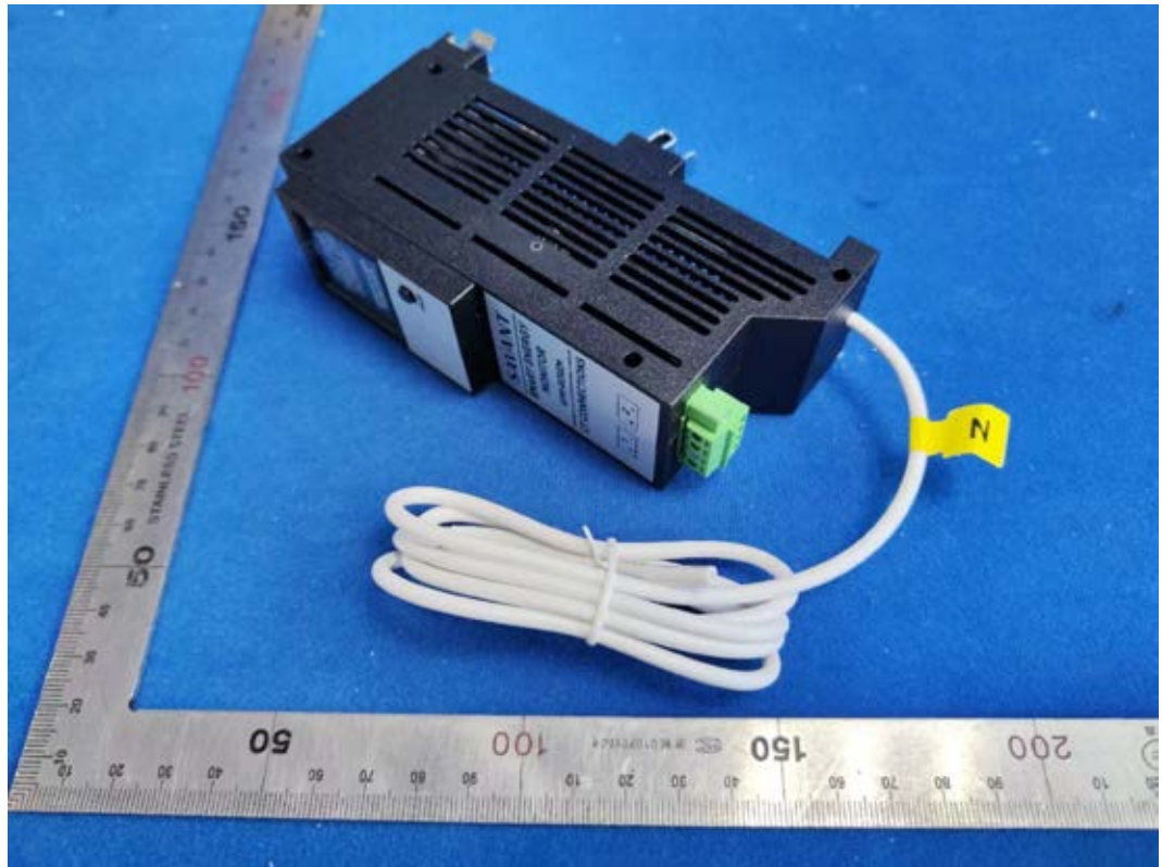
FIGURE 8 QO 2-CHANNEL POWER MONITOR MODULE, PIGTAIL (M/N: GPM-Q2SEM-00) GENERAL APPEARANCE FRONT VIEW
