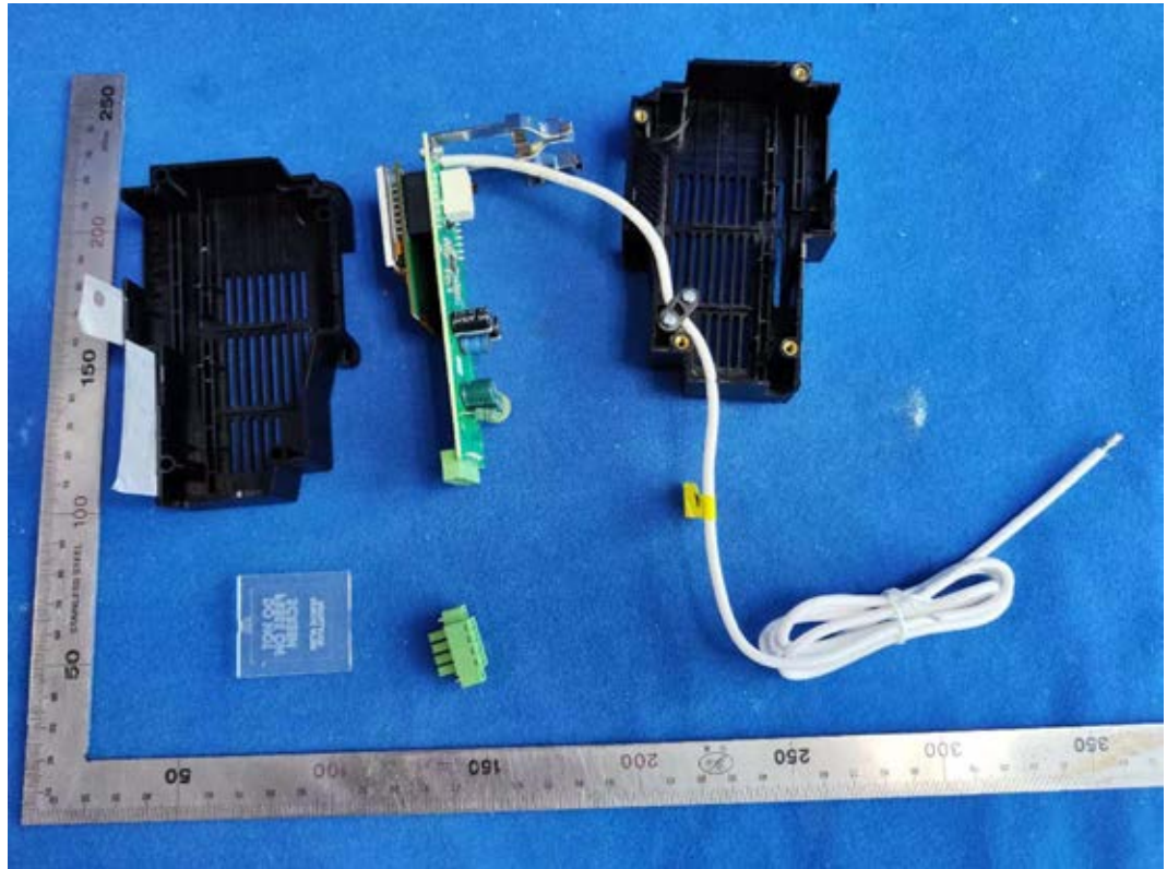
FIGURE 1 1-INCH 2-CHANNEL POWER MONITOR MODULE, PIGTAIL (M/N: GPM-H2SEM-00) COVER REMOVED
