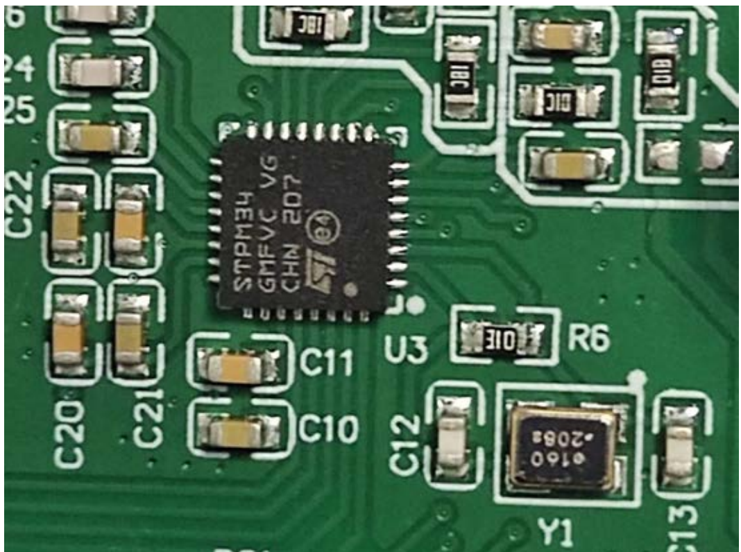
FIGURE 4 1-INCH 2-CHANNEL POWER MONITOR MODULE, PIGTAIL (M/N: GPM-H2SEM-00) CHIP AND CRYSTAL ON POWER BOARD
