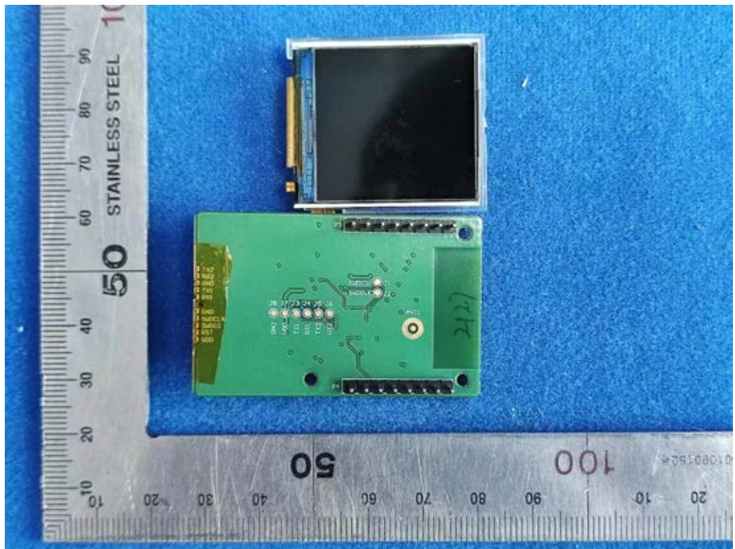
FIGURE 6 1-INCH 2-CHANNEL POWER MONITOR MODULE, PIGTAIL (M/N: GPM-H2SEM-00) RF BOARD BACK VIEW
