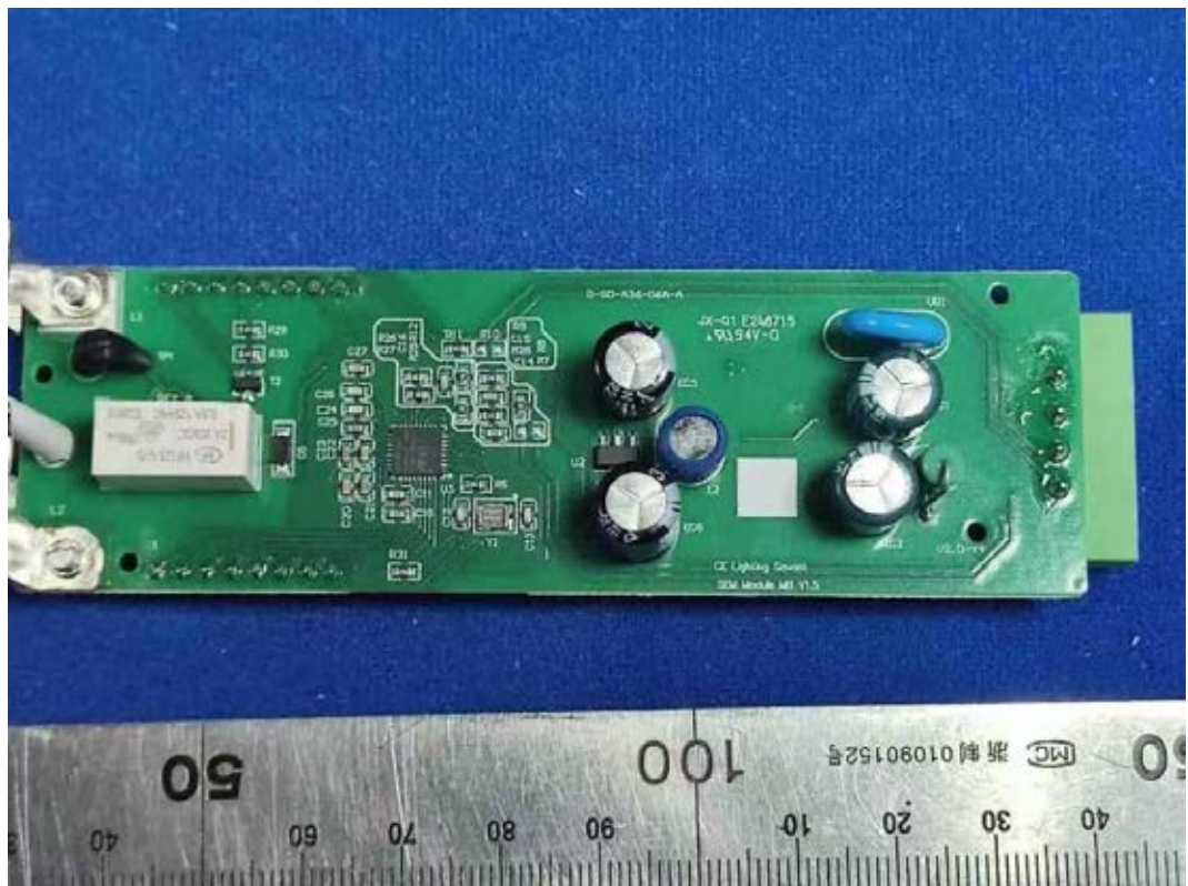
FIGURE 2 1-INCH 2-CHANNEL POWER MONITOR MODULE, PIGTAIL (M/N: GPM-H2SEM-00) POWER BOARD FRONT VIEW
