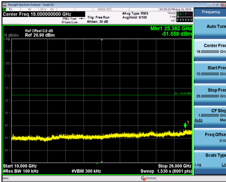
RF Conducted Spurious Emissions_11N40SISO_2452_Ant1
