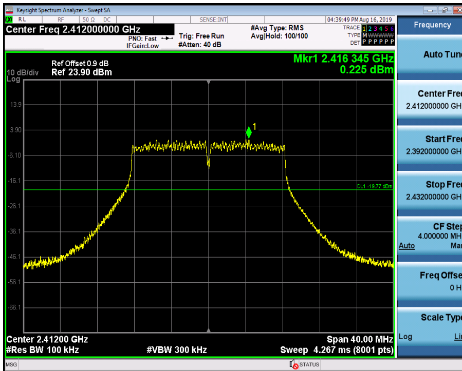
RF Conducted Spurious Emissions_11G_2412_Ant1
