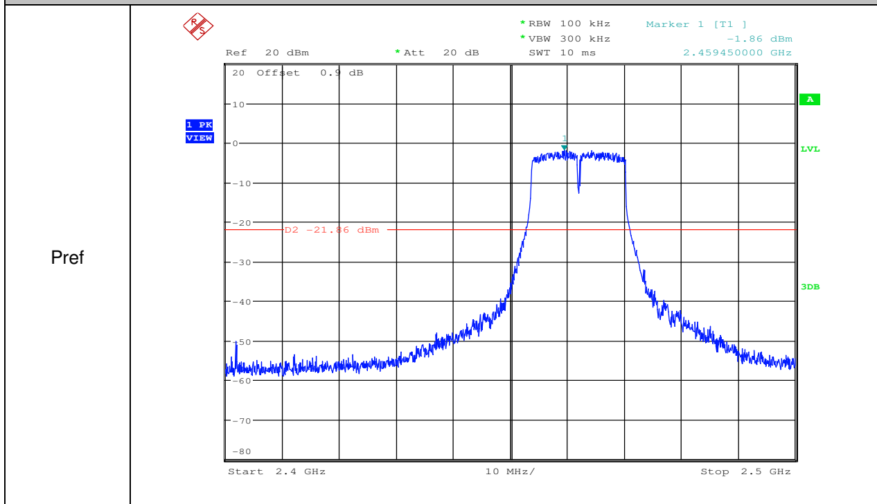
RF Conducted Spurious Emissions_11G_2462_Ant1
