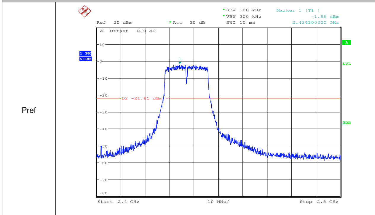
RF Conducted Spurious Emissions_11N20SISO_2437_Ant1
