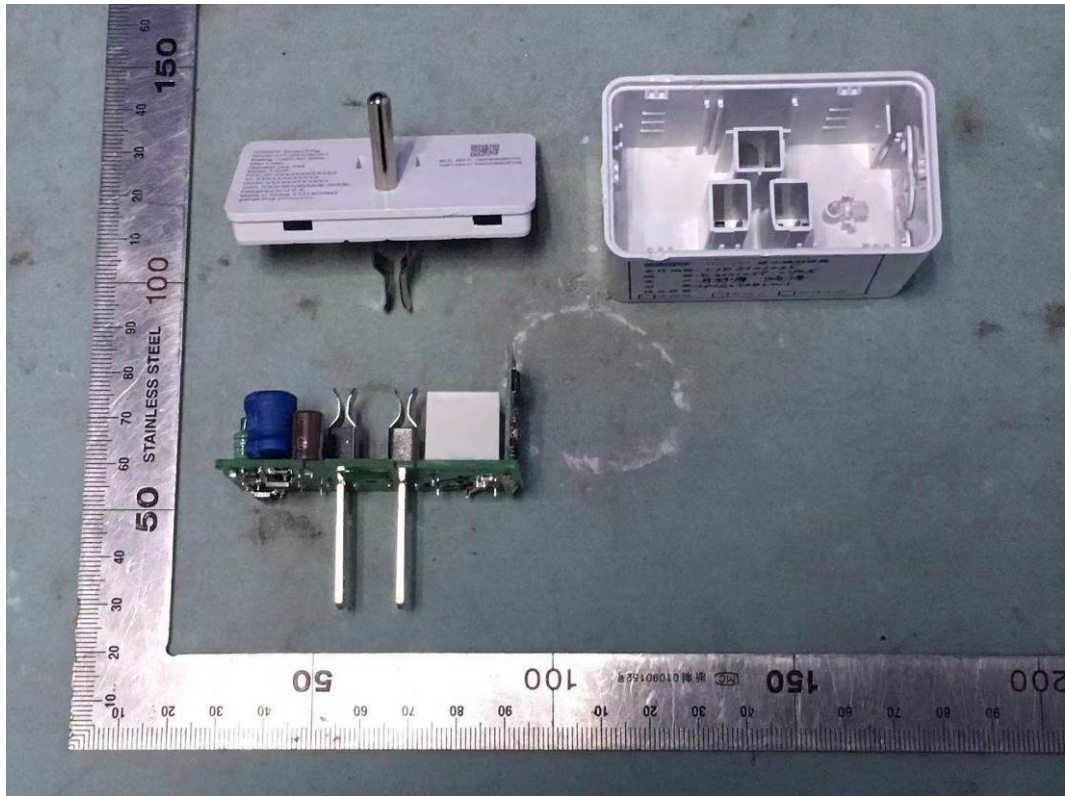
FIGURE 2 SMART PLUG (M/N: CPLGSTDBLW1) MAIN BOARD (COMPONENT SIDE)
