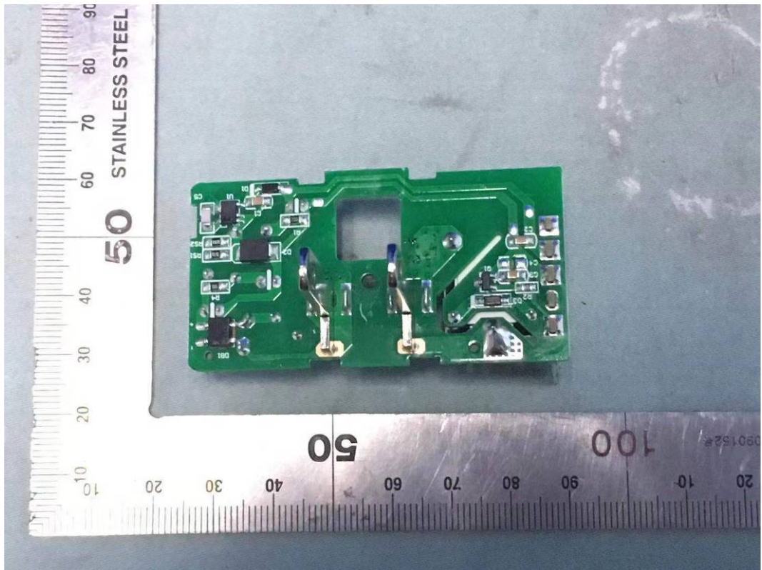
FIGURE 3 SMART PLUG (M/N: CPLGSTDBLW1) MAIN BOARD (SOLDERED SIDE)
