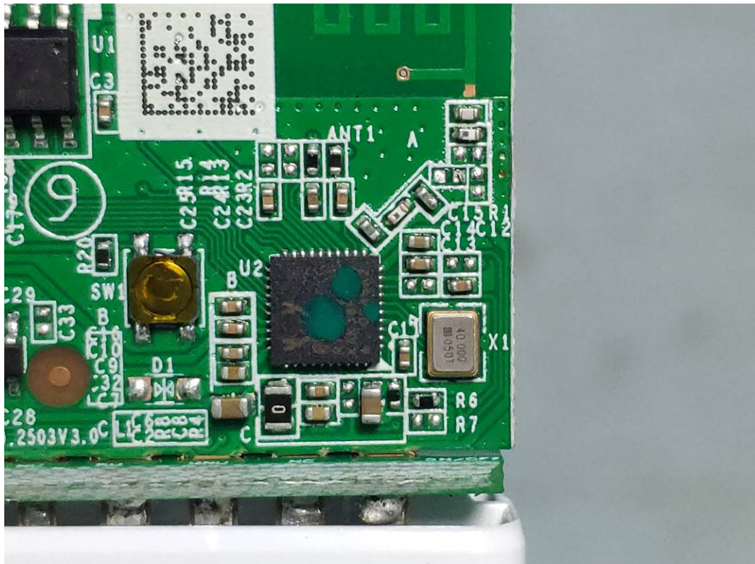
FIGURE 5 SMART PLUG (M/N: CPLGSTDBLW1) CHIP & CRYSTAL ON RF BOARD (GENERAL VIEW)
