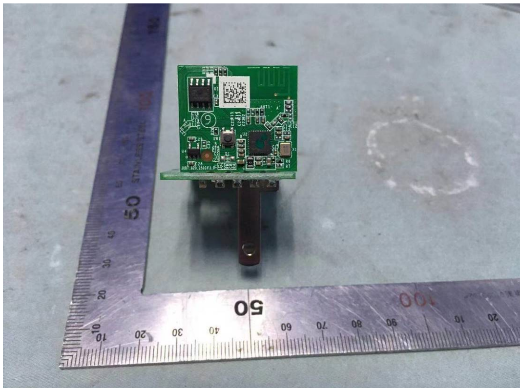
FIGURE 4 SMART PLUG (M/N: CPLGSTDBLW1) RF BOARD (COMPONENT SIDE)
