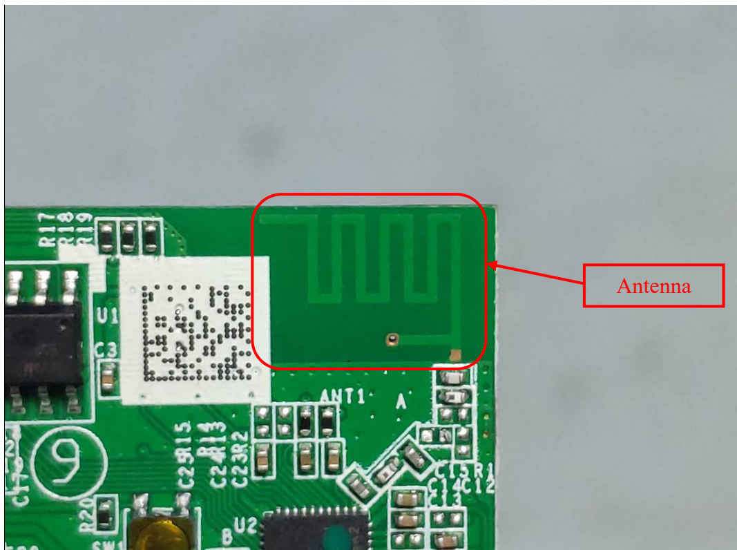
FIGURE 6 SMART PLUG (M/N: CPLGSTDBLW1) ANTENNA (GENERAL VIEW)
