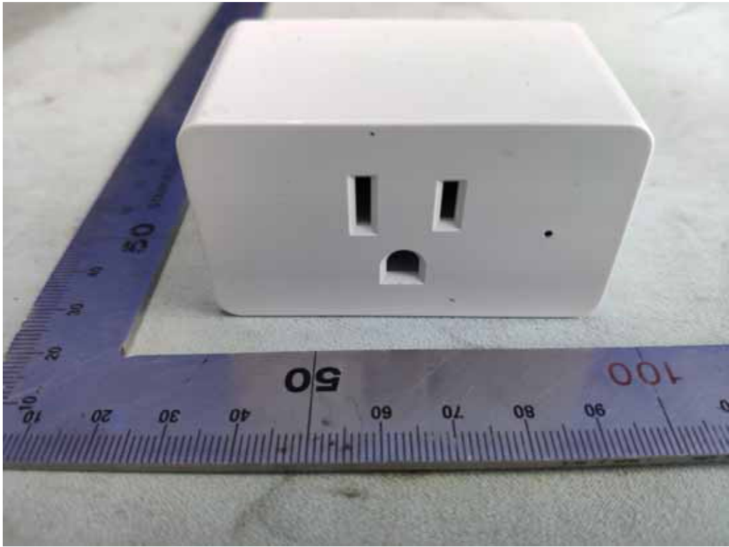
FIGURE 3 SMART PLUG (M/N: CPLGSTDBLW1) GENERAL APPEARANCE (FRONT VIEW)
