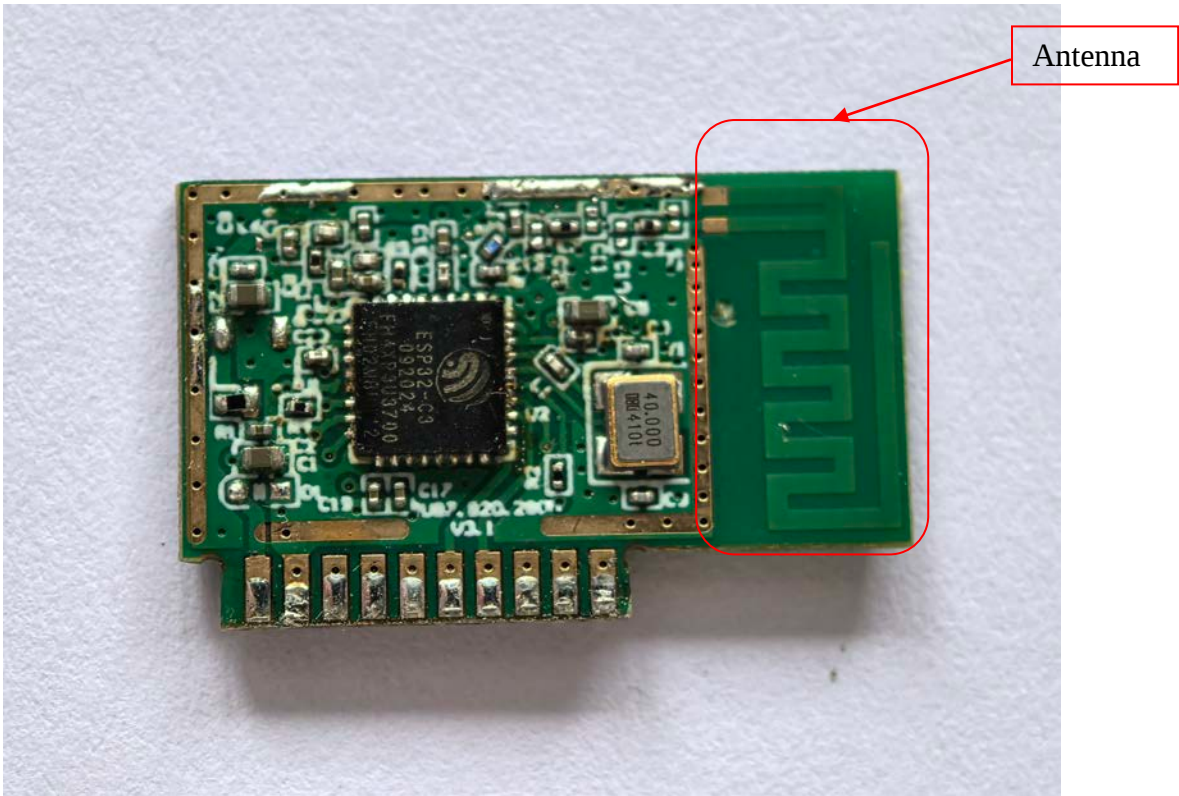
FIGURE 12 ON/OFF SMART PLUG (M/N: CPLGSTDBLW1MS) CHIP&CRYSTAL ON BOARD
