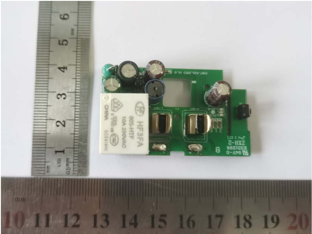
FIGURE 8 ON/OFF SMART PLUG (M/N: CPLGSTDBLW1MS) MAINBOARD FRONT
