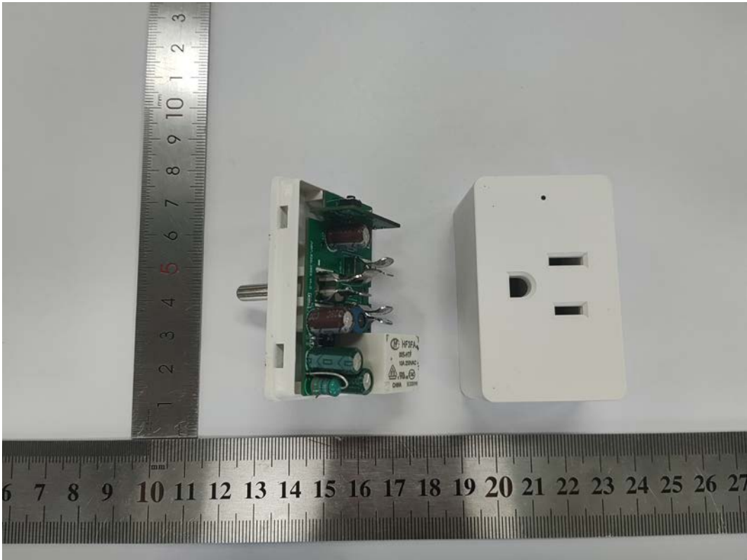
FIGURE 7 ON/OFF SMART PLUG (M/N: CPLGSTDBLW1MS) COVER REMOVED
