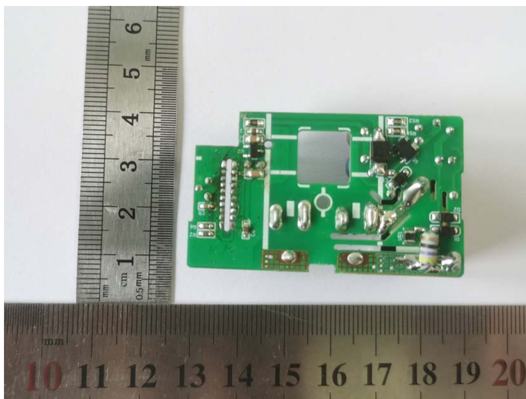
FIGURE 9 ON/OFF SMART PLUG (M/N: CPLGSTDBLW1MS) MAINBOARD BACK
