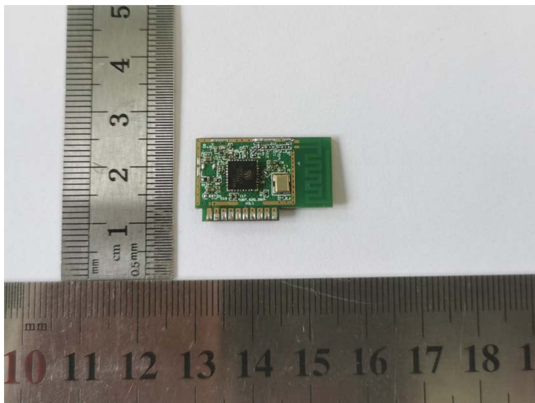
FIGURE 10 ON/OFF SMART PLUG (M/N: CPLGSTDBLW1MS) RFBOARD FRONT
