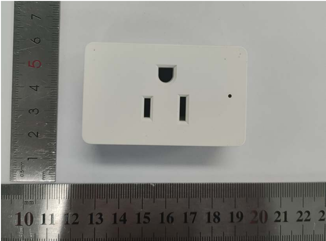
FIGURE 1 ON/OFF SMART PLUG (M/N: CPLGSTDBLW1MS) GENERAL VIEW
