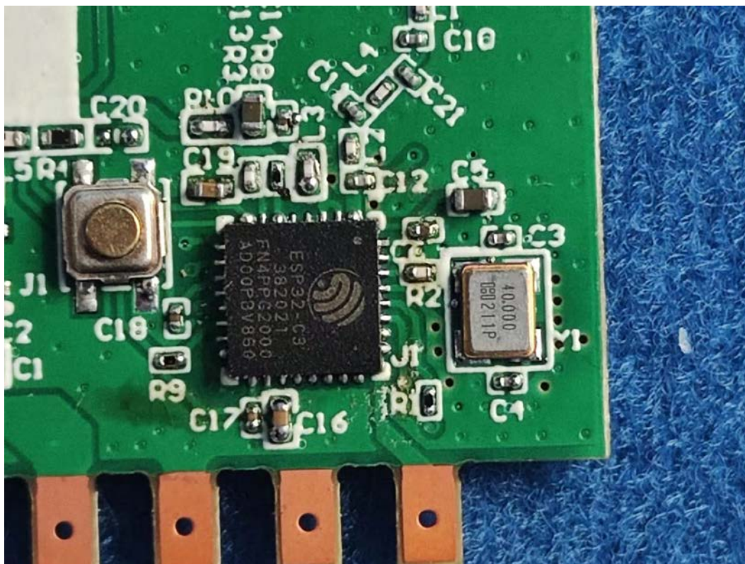
FIGURE 8 SMART PLUG (M/N: CPLGSTDBLW1) CHIP & CRYSTAL ON RF BOARD
