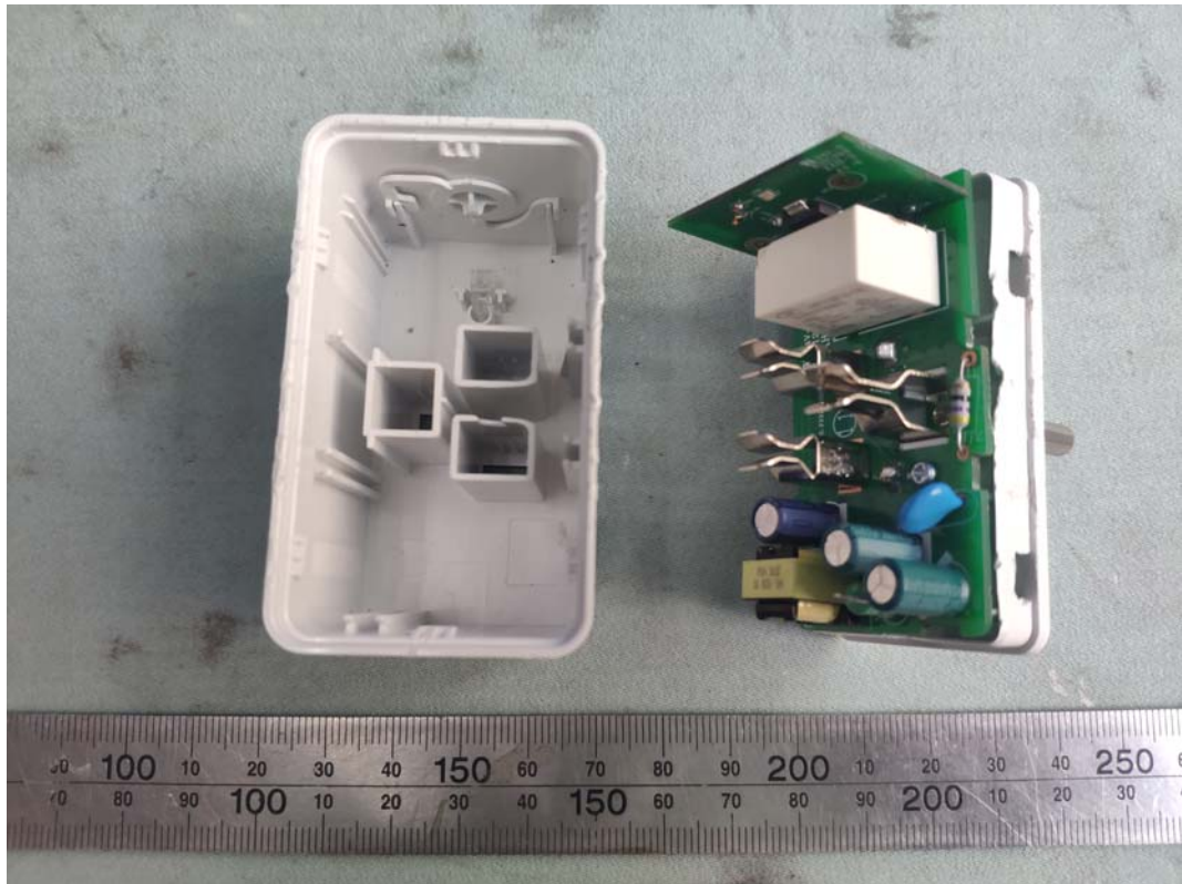
FIGURE 7 SMART PLUG (MODEL: CPLGSTDBLW1)(HVIN: CPLGSTDXCWIT) COVER REMOVED
