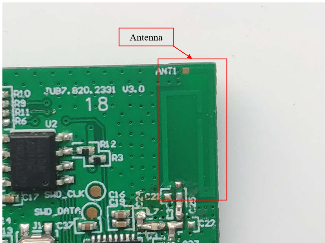
FIGURE 14 SMART PLUG (MODEL: CPLGSTDBLW1)(HVIN: CPLGSTDXCWIT) WLAN ANT
