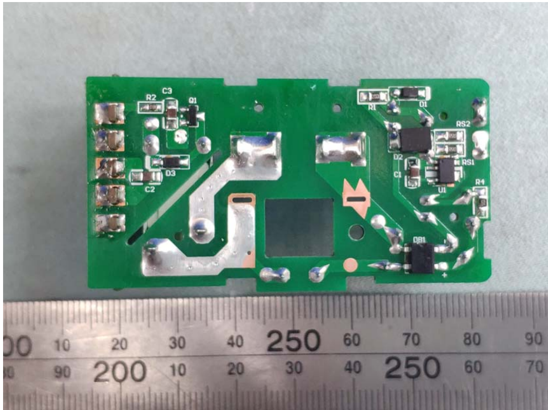
FIGURE 9 SMART PLUG (MODEL: CPLGSTDBLW1)(HVIN: CPLGSTDXCWIT) MAIN BOARD (SOLDERED SIDE)
