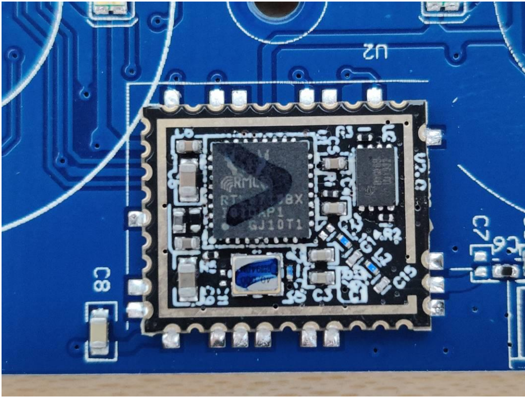
Detail view of WIFI module
