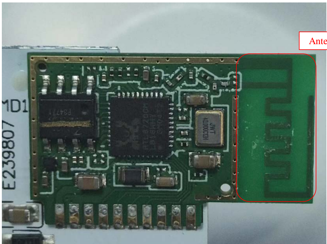
FIGURE 10 DOWNLIGHT (M/N: CFIXCNLR6SD) CHIP & CRYSTAL ON BOARD
