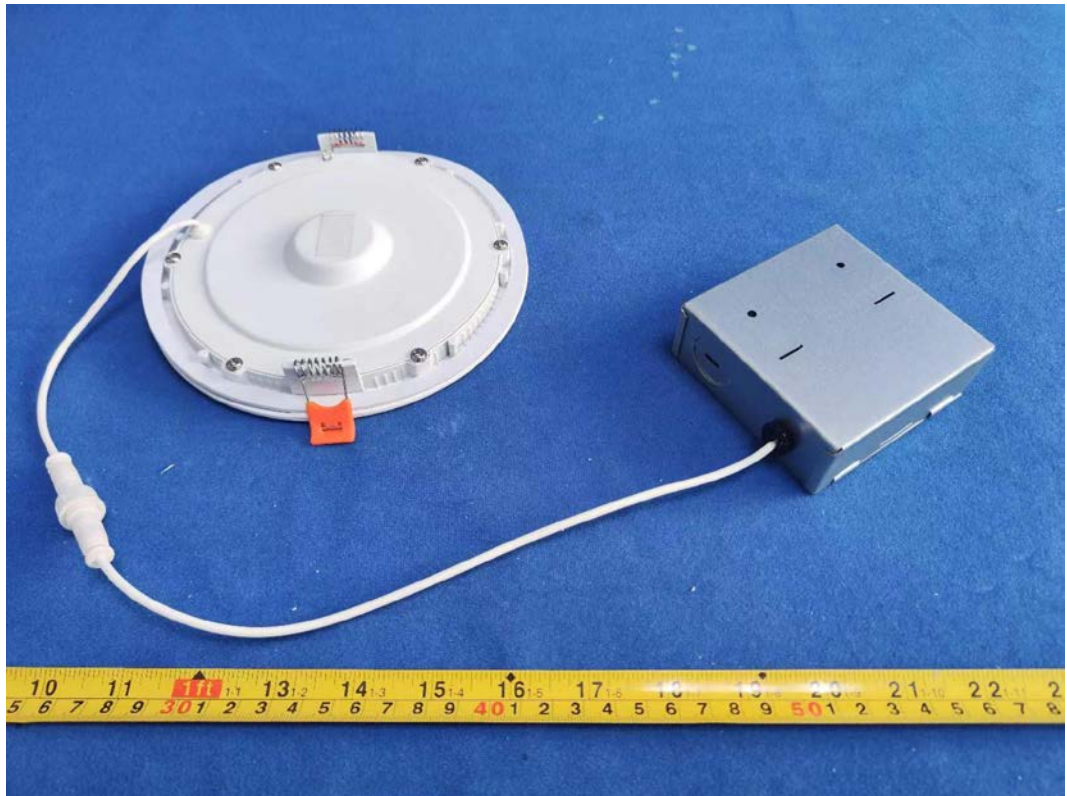
FIGURE 4 DOWNLIGHT (M/N: CFIXCNLR6C1) BACK VIEW
