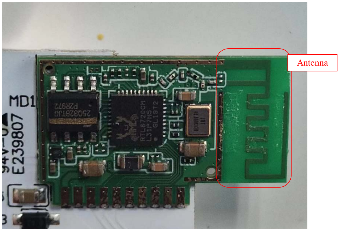
FIGURE 17 DOWNLIGHT (M/N: CFIXCNLR4S1) CHIP & CRYSTAL ON BOARD
