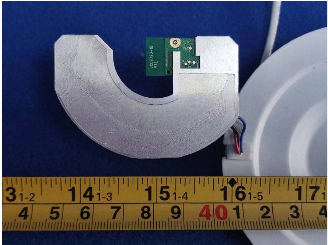
FIGURE 16 DOWNLIGHT (M/N: CFIXCNLR4S1) MAIN BOARD (SOLDERED SIDE)
