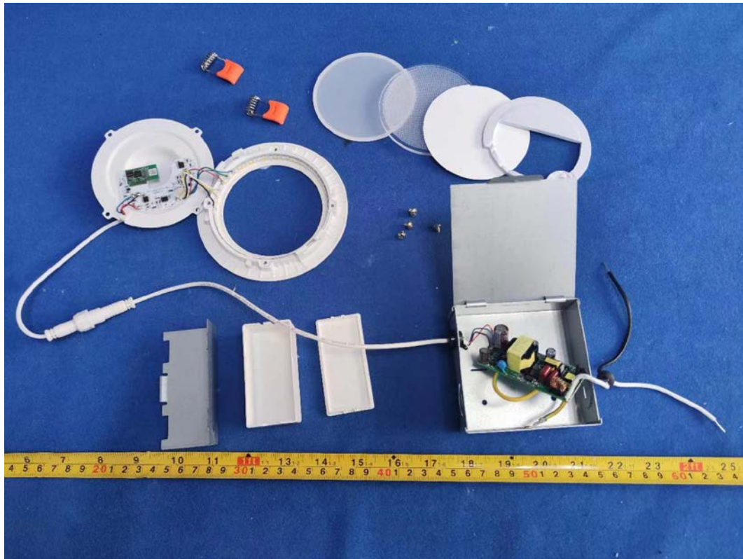
FIGURE 12 DOWNLIGHT (M/N: CFIXCNLR4S1) COVER REMOVED
