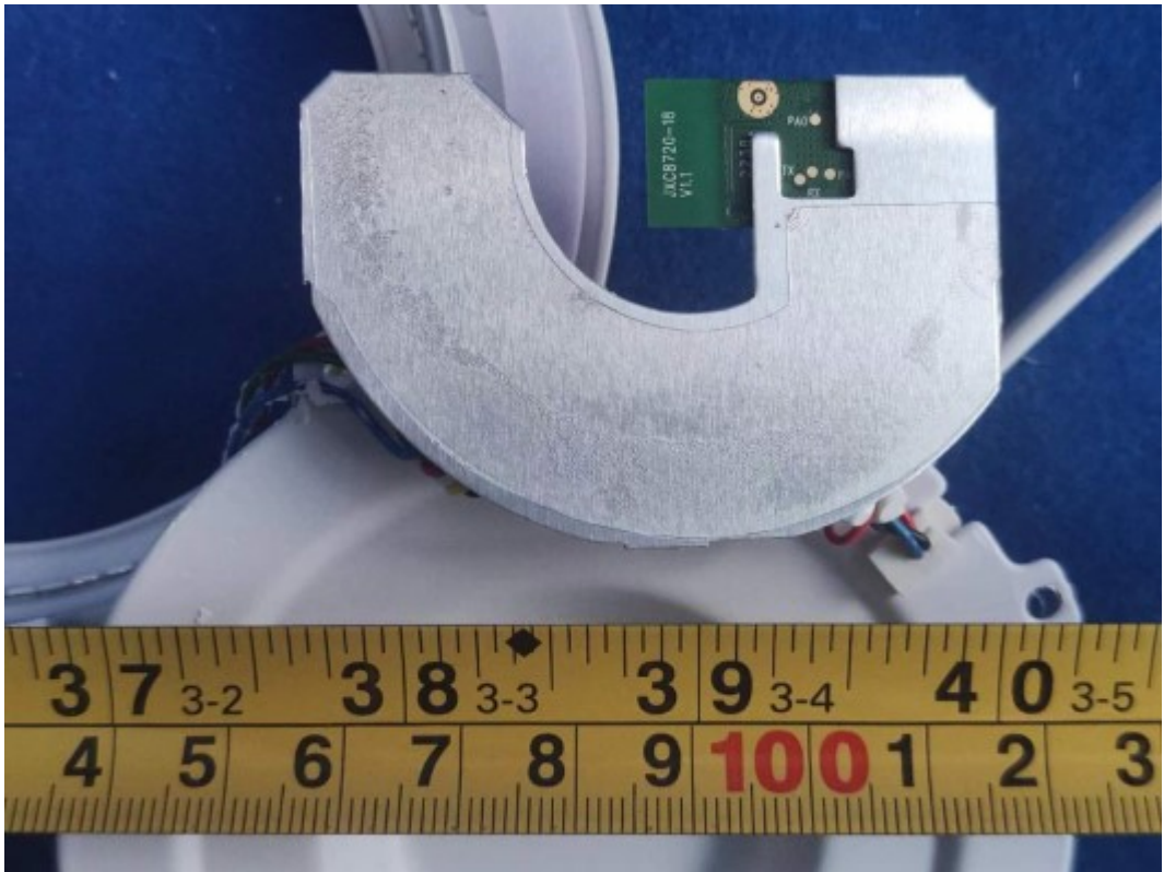
FIGURE 9 DOWNLIGHT (M/N: CFIXCNLR4SD) MAIN BOARD (SOLDERED SIDE)
