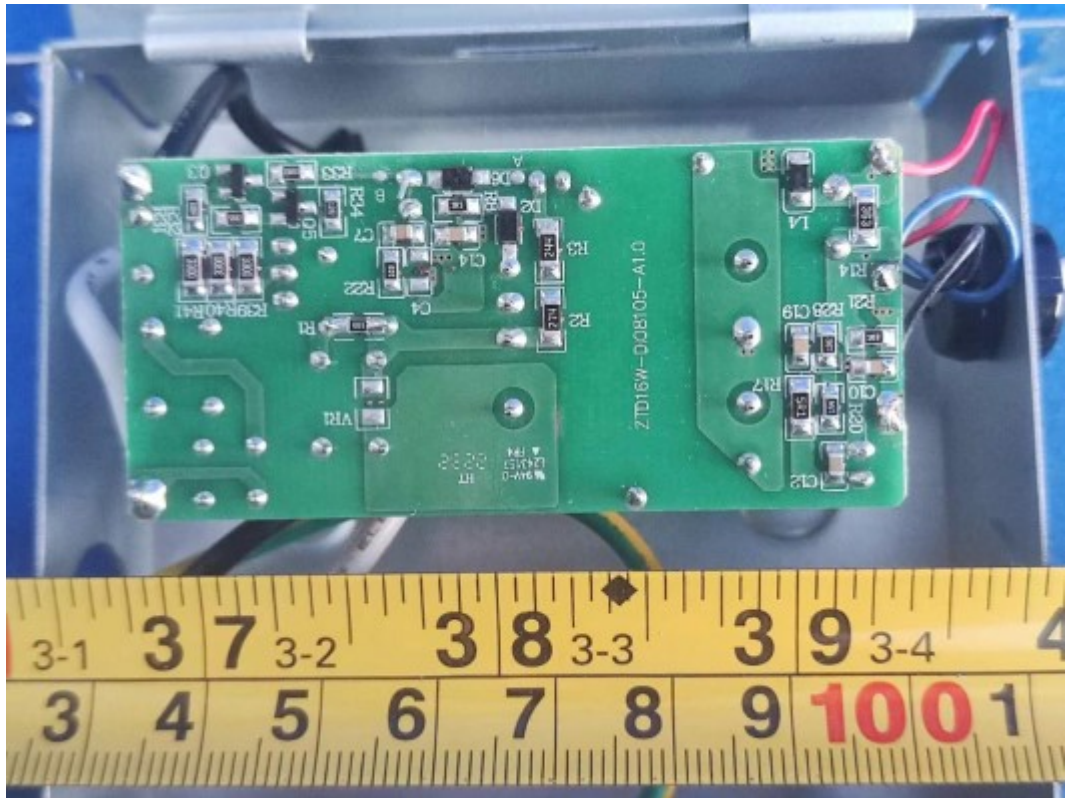
FIGURE 7 DOWNLIGHT (M/N: CFIXCNLR4SD) POWER BOARD (SOLDERED SIDE)
