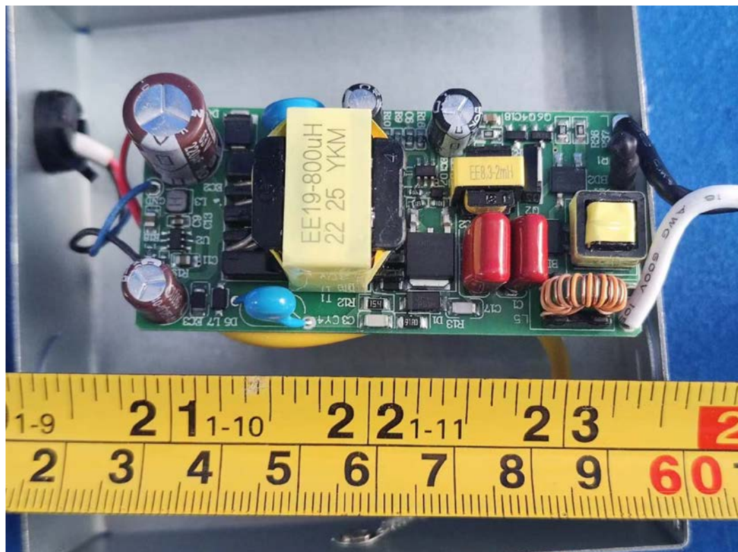
FIGURE 13 DOWNLIGHT (M/N: CFIXCNLR4S1) POWER BOARD (COMPONENT SIDE)
