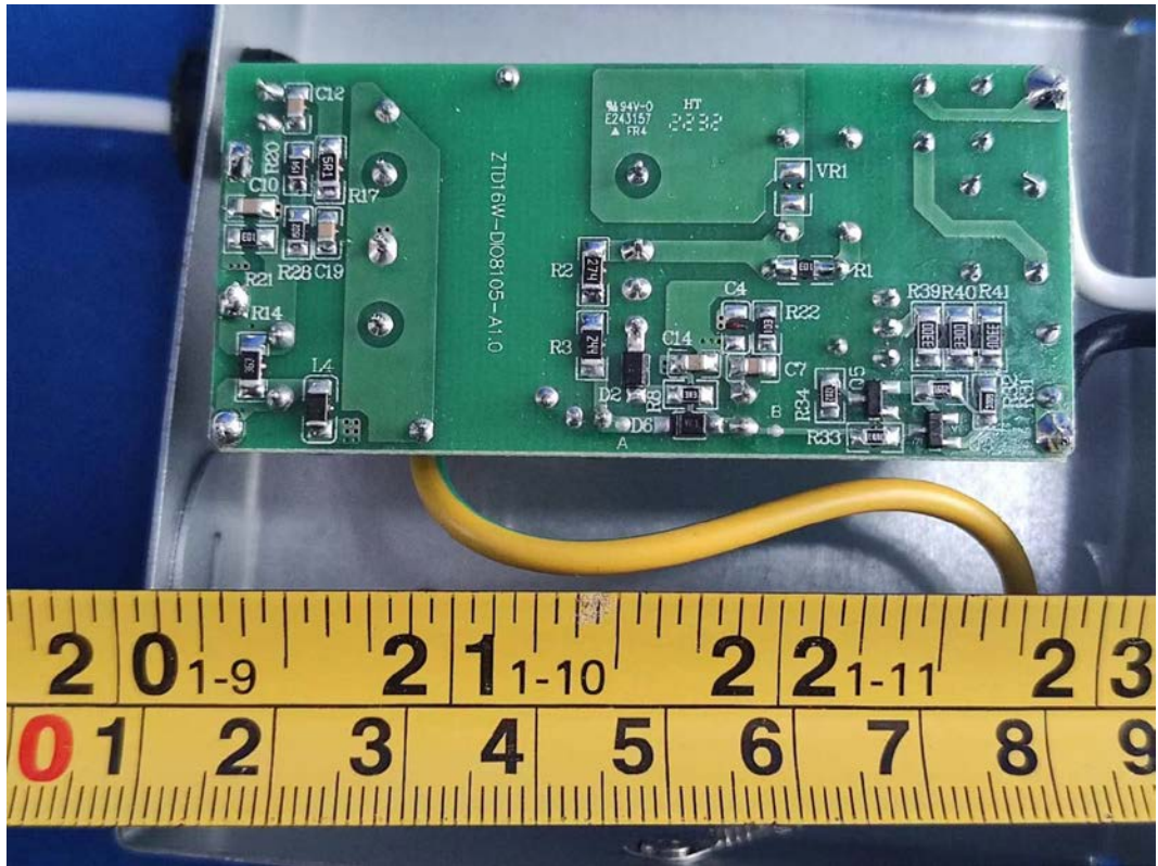
FIGURE 14 DOWNLIGHT (M/N: CFIXCNLR4S1) POWER BOARD (SOLDERED SIDE)
