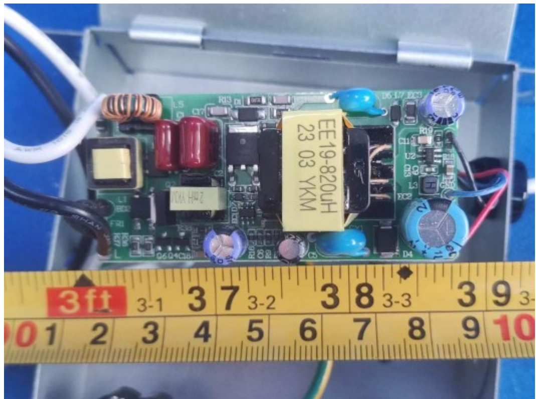
FIGURE 6 DOWNLIGHT (M/N: CFIXCNLR4SD) POWER BOARD (COMPONENT SIDE)
