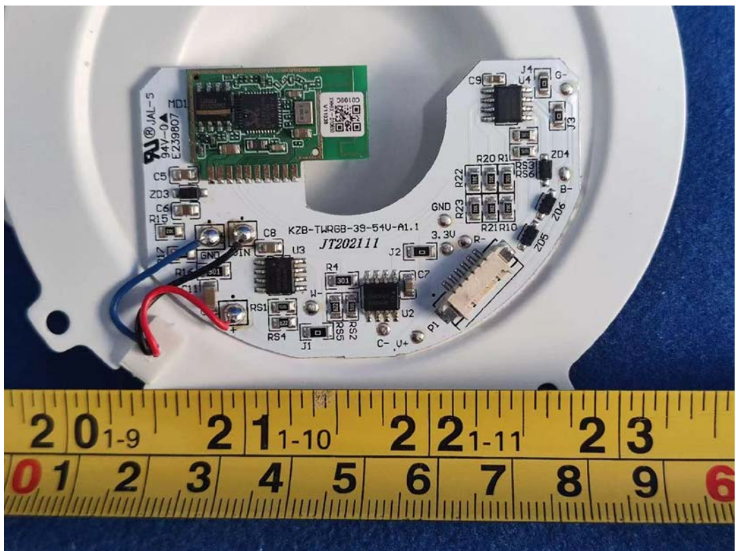
FIGURE 15 DOWNLIGHT (M/N: CFIXCNLR4S1) MAIN BOARD (COMPONENT SIDE)
