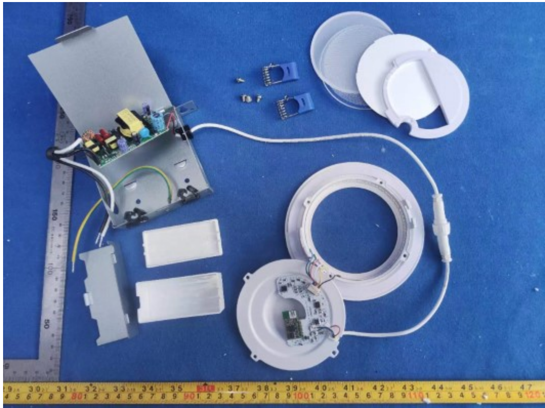
FIGURE 5 DOWNLIGHT (M/N: CFIXCNLR4SD) COVER REMOVED
