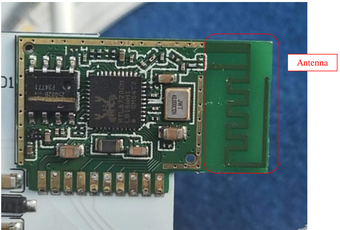
FIGURE 10 DOWNLIGHT (M/N: CFIXCNLR4SD) CHIP & CRYSTAL ON BOARD
