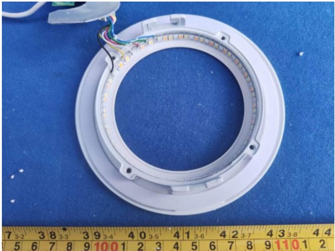
FIGURE 11 DOWNLIGHT (M/N: CFIXCNLR4SD) LED
