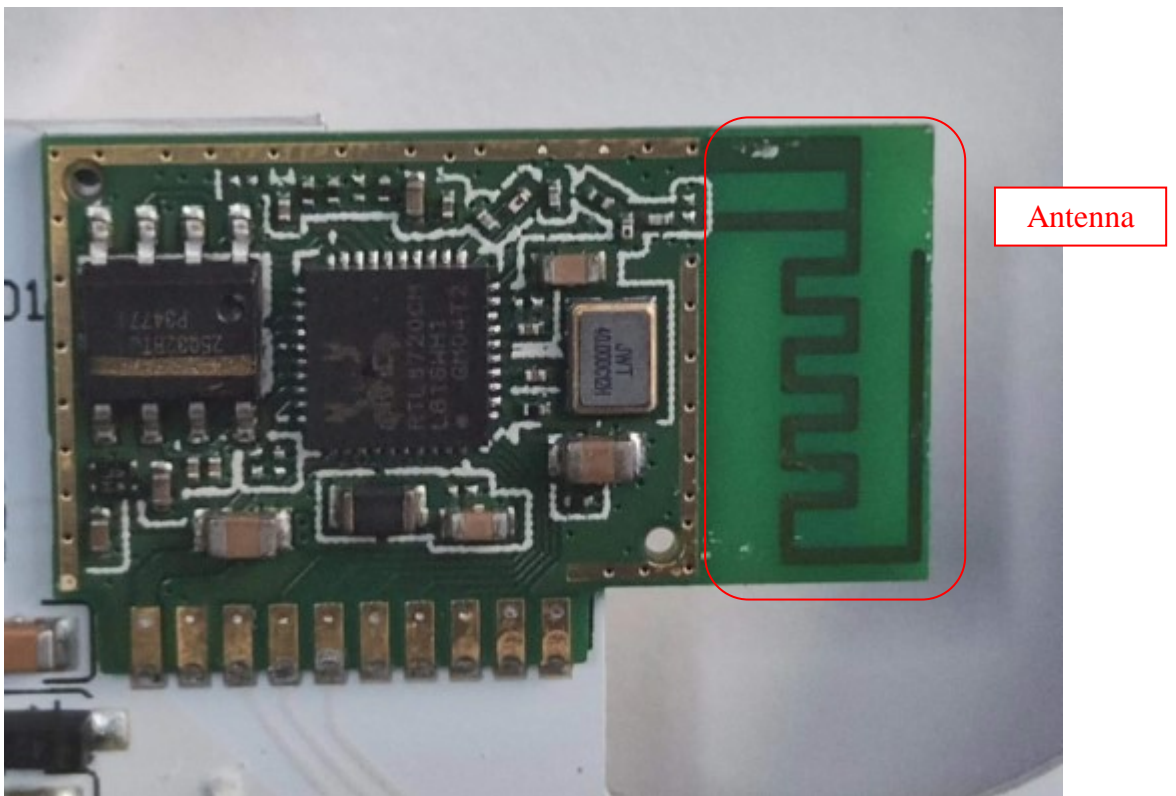
FIGURE 10 DOWNLIGHT (M/N: CFIXCNLR4CRVD) CHIP & CRYSTAL ON BOARD
