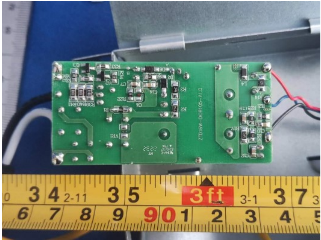
FIGURE 7 DOWNLIGHT (M/N: CFIXCNLR4CRVD) POWER BOARD (SOLDERED SIDE)
