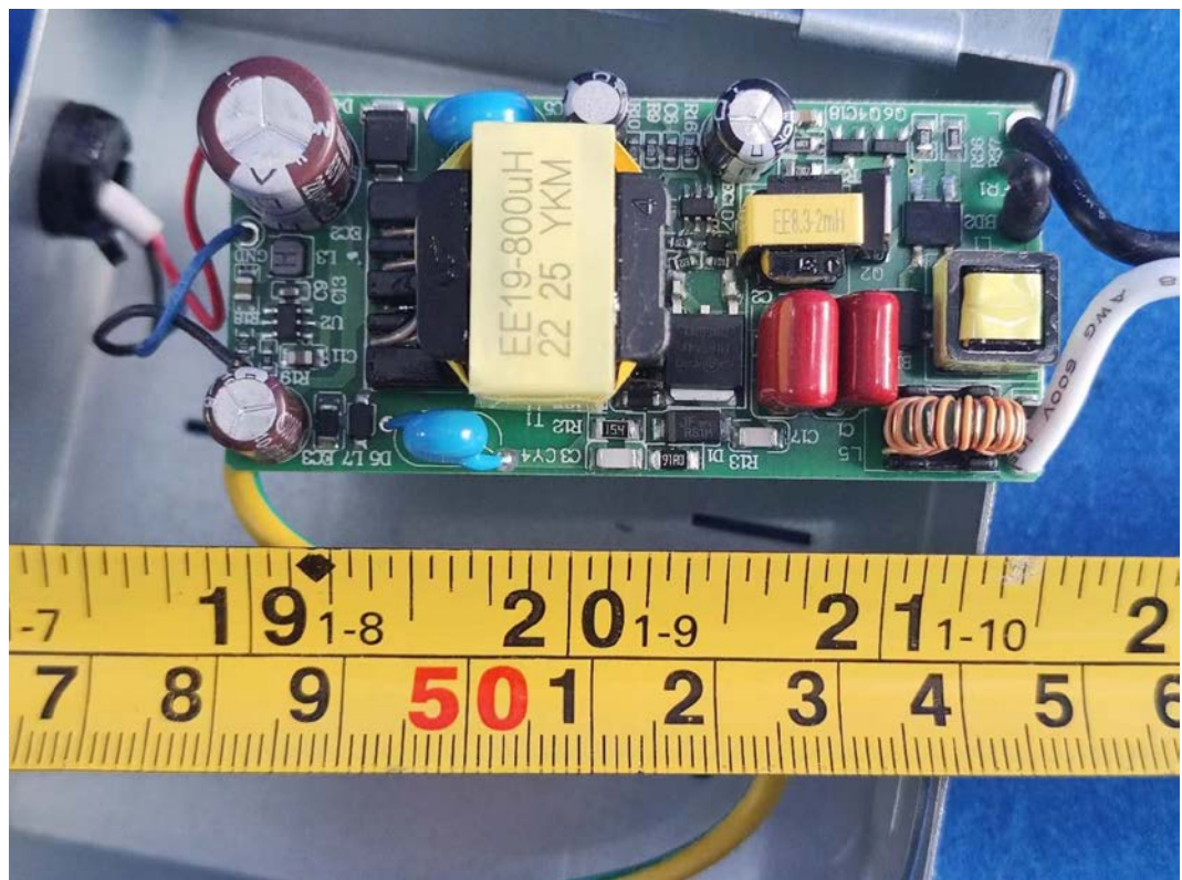
FIGURE 13 DOWNLIGHT (M/N: CFIXCNLR4C1) POWER BOARD (COMPONENT SIDE)
