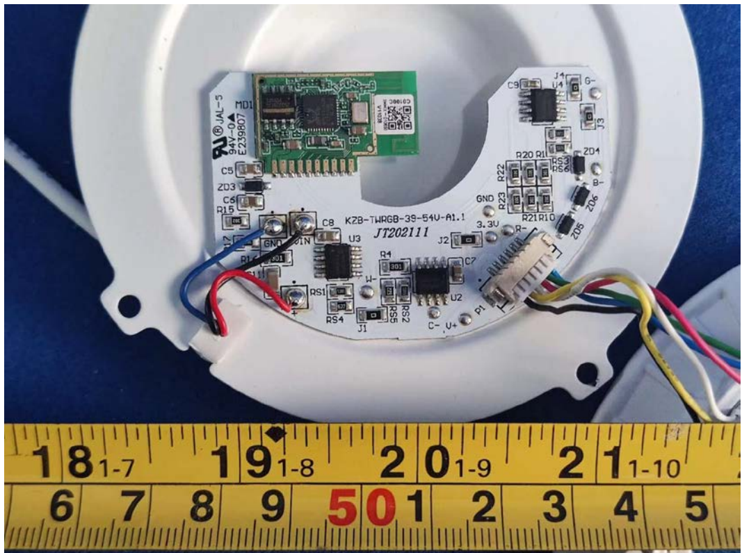
FIGURE 15 DOWNLIGHT (M/N: CFIXCNLR4C1) MAIN BOARD (COMPONENT SIDE)
