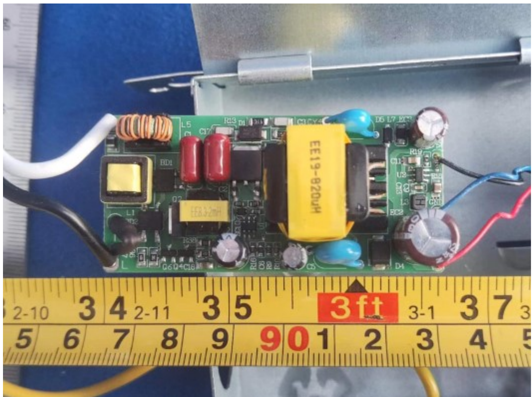
FIGURE 6 DOWNLIGHT (M/N: CFIXCNLR4CRVD) POWER BOARD (COMPONENT SIDE)
