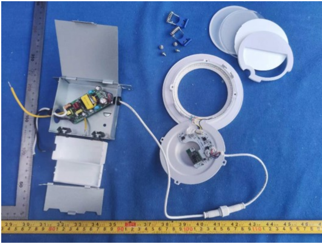
FIGURE 5 DOWNLIGHT (M/N: CFIXCNLR4CRVD) COVER REMOVED
