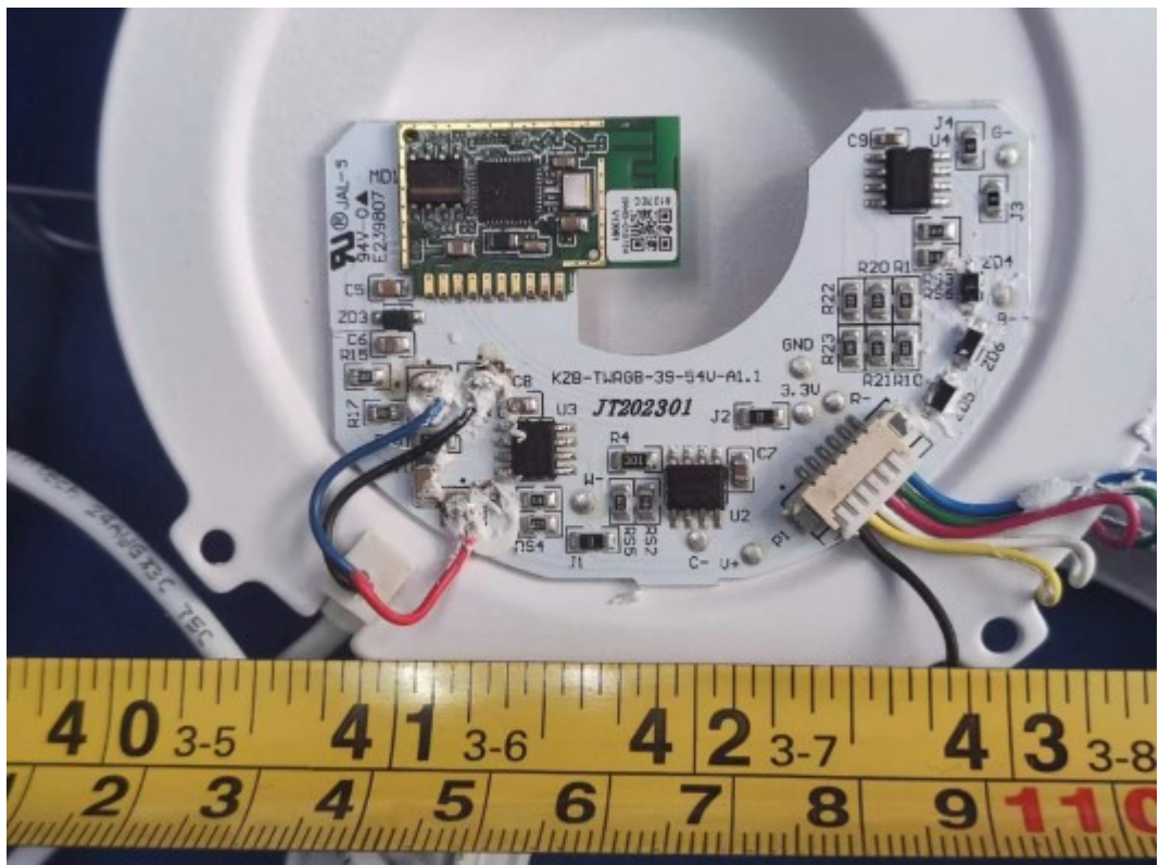
FIGURE 8 DOWNLIGHT (M/N: CFIXCNLR4CRVD) MAIN BOARD (COMPONENT SIDE)
