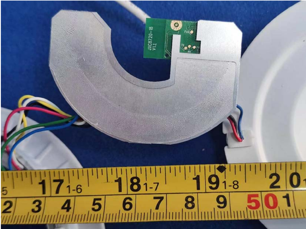
FIGURE 16 DOWNLIGHT (M/N: CFIXCNLR4C1) MAIN BOARD (SOLDERED SIDE)
