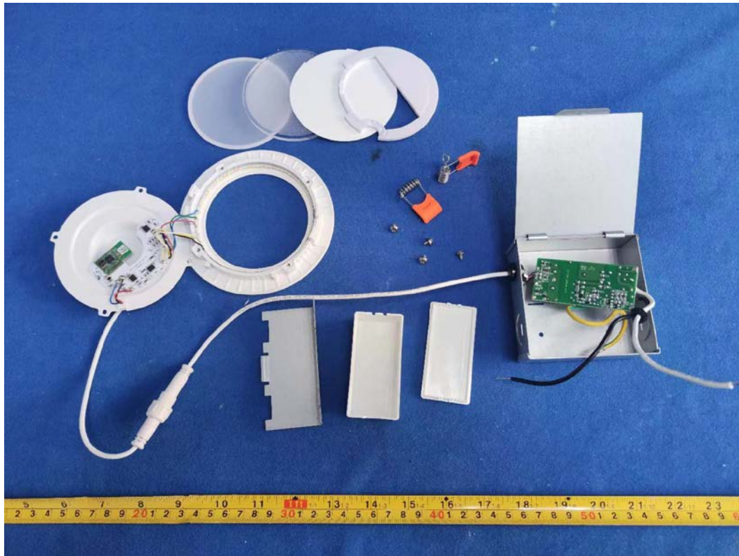
FIGURE 12 DOWNLIGHT (M/N: CFIXCNLR4C1) COVER REMOVED
