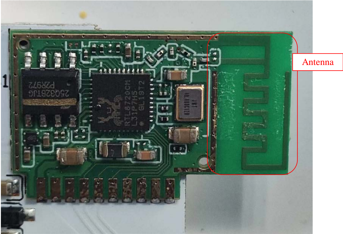
FIGURE 17 DOWNLIGHT (M/N: CFIXCNLR4C1) CHIP & CRYSTAL ON BOARD
