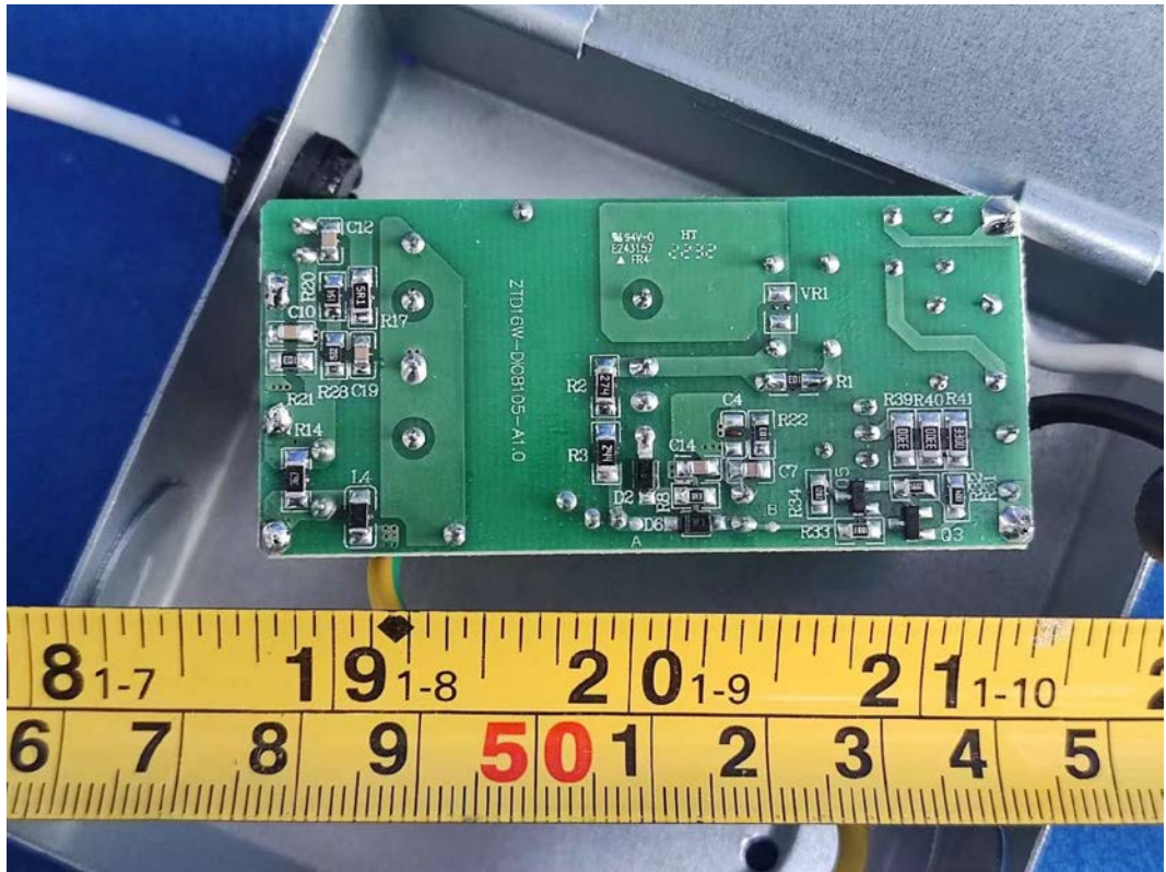
FIGURE 14 DOWNLIGHT (M/N: CFIXCNLR4C1) POWER BOARD (SOLDERED SIDE)
