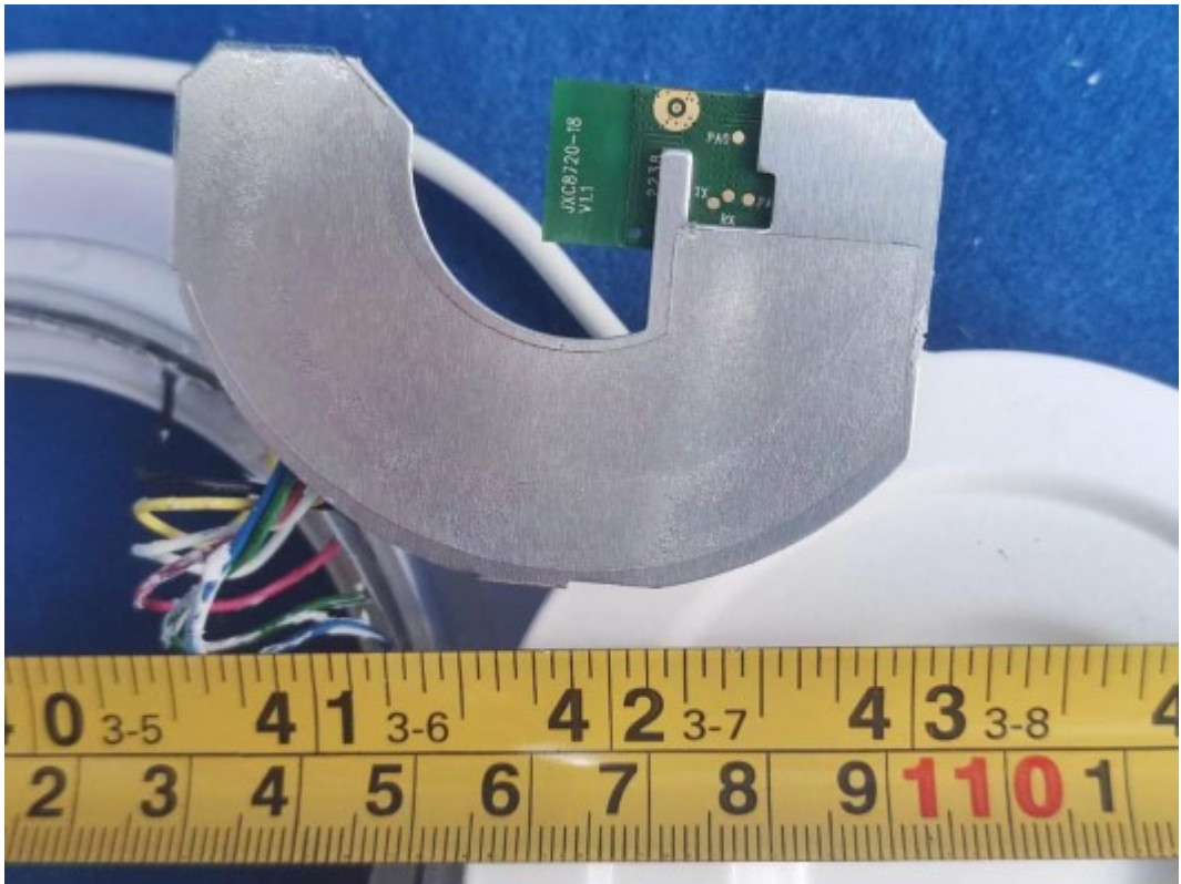
FIGURE 9 DOWNLIGHT (M/N: CFIXCNLR4CRVD) MAIN BOARD (SOLDERED SIDE)
