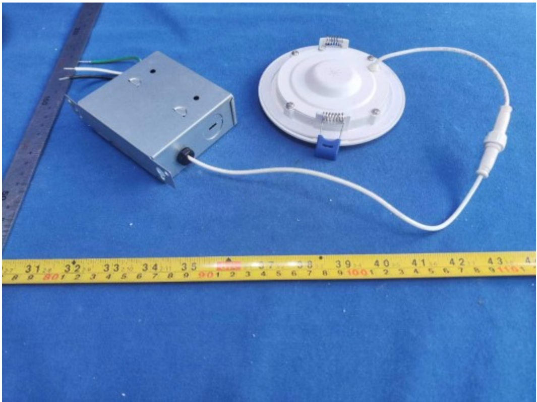
FIGURE 2 DOWNLIGHT (M/N: CFIXCNLR4CRVD) BACK VIEW
