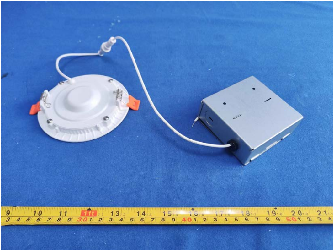
FIGURE 4 DOWNLIGHT (M/N: CFIXCNLR4C1) BACK VIEW
