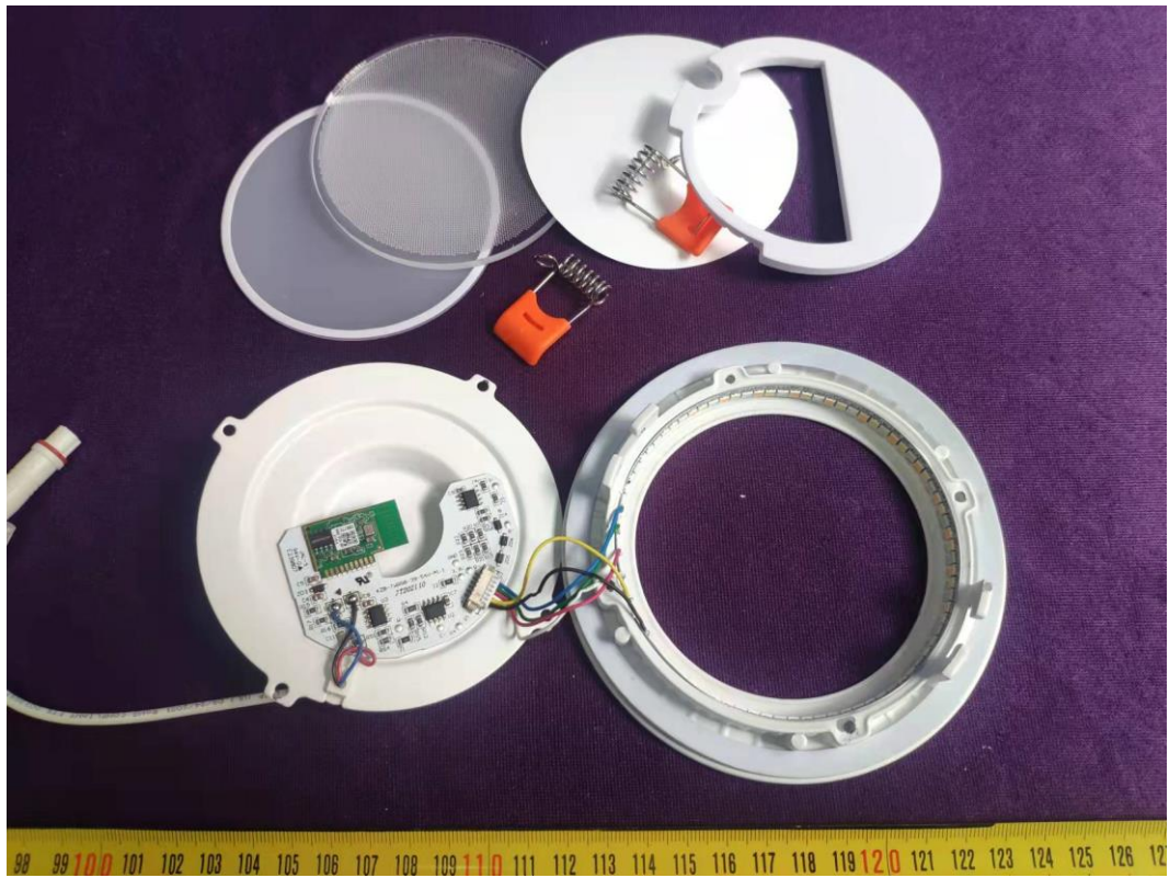
FIGURE 8 CYNCR FIXTURE CANLESS (M/N: CFIXCNLR4C1) LED
