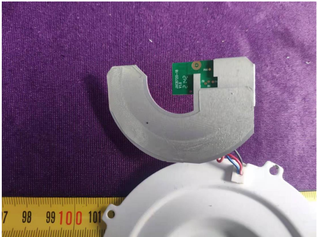
FIGURE 4 CYNCR FIXTURE CANLESS (M/N: CFIXCNLR4C1) CHIP & CRYSTAL ON BOARD
