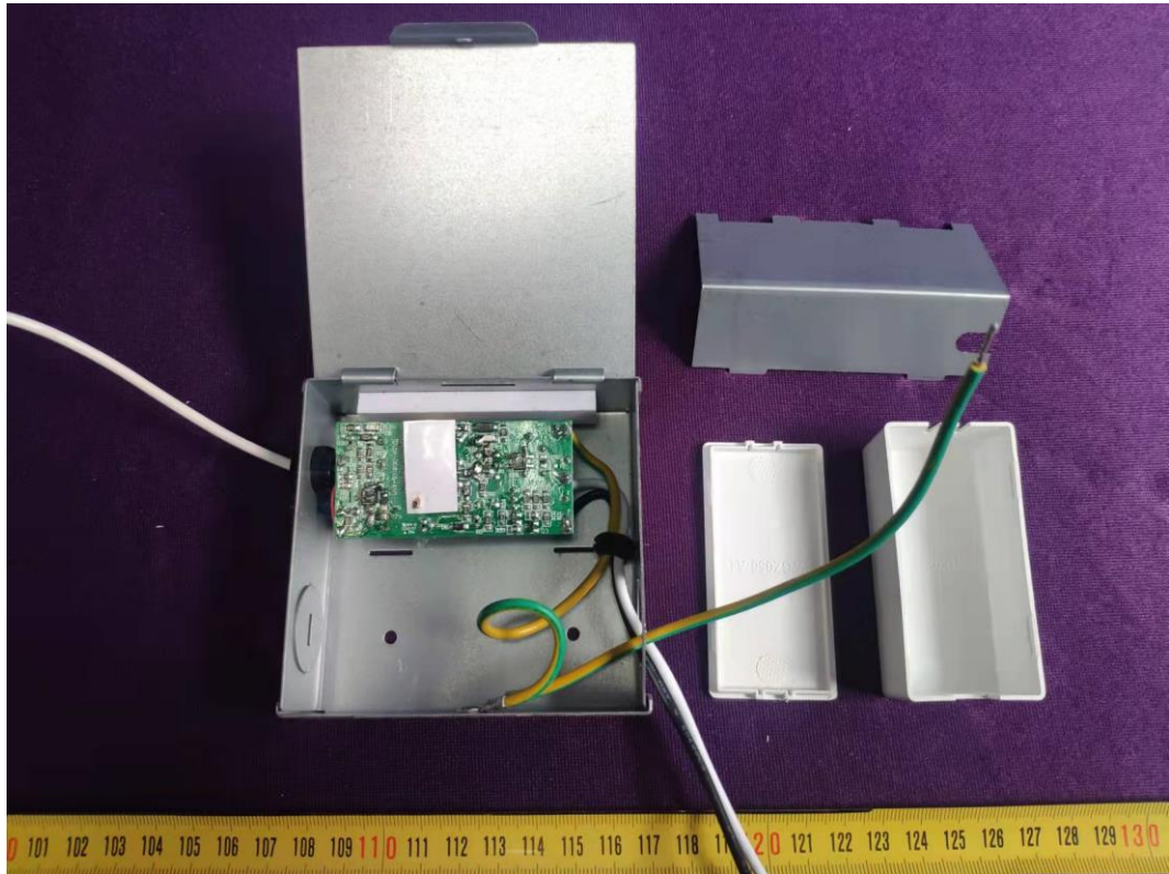
FIGURE 2 CYNX FIXTURE CANLESS (M/N: CFIXCNLR4C1) MAIN BOARD (COMPONENT SIDE)
