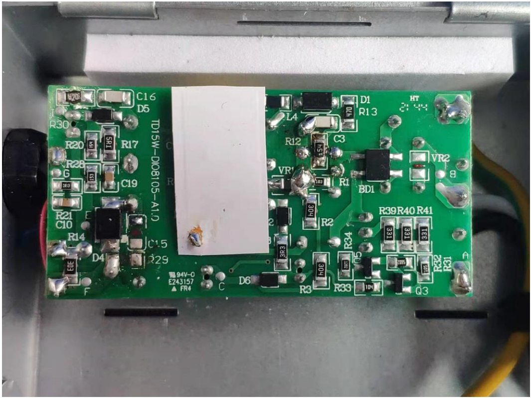
FIGURE 6 CYNC FIXTURE CANLESS (M/N: CFIXCNLR4C1) POWER BOARD (SOLDERED SIDE)
