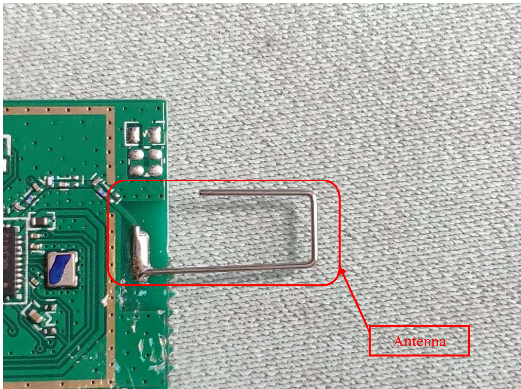
FIGURE 5 DUAL MODE TUNABLE WHITE BR30 (M/N: CLEDR309SD1) ANTENNA
