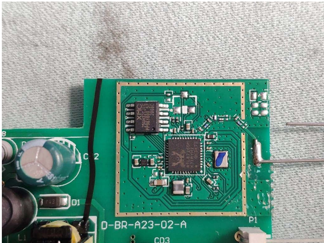
FIGURE 4 DUAL MODE TUNABLE WHITE BR30 (M/N: CLEDR309SD1) CHIP & CRYSTAL ON BOARD
