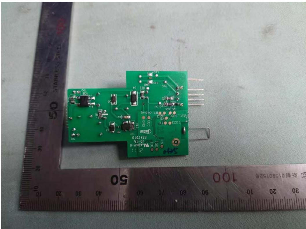
FIGURE 3 DUAL MODE TUNABLE WHITE BR30 (M/N: CLEDR309SD1) MAIN BOARD (SOLDERED SIDE)
