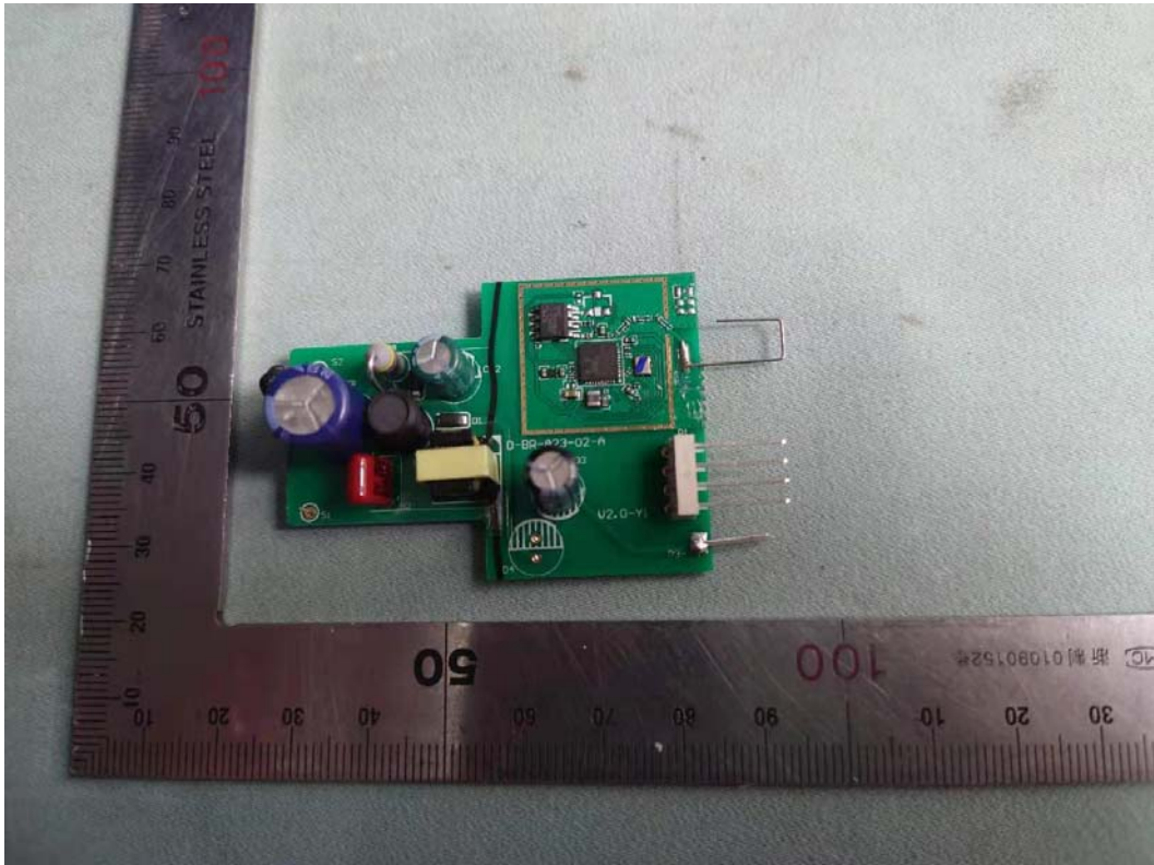
FIGURE 2 DUAL MODE TUNABLE WHITE BR30 (M/N: CLEDR309SD1) MAIN BOARD (COMPONENT SIDE)
