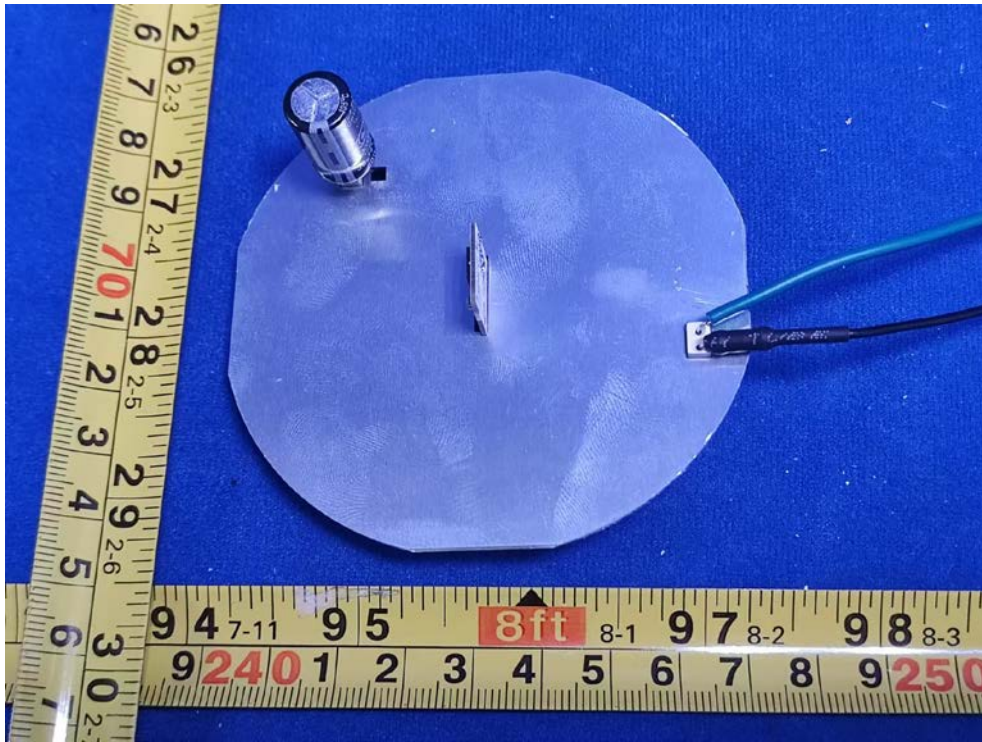
FIGURE 10 DIRECT CONNECT FULL COLOR BR30 (M/N: CLEDR309CD1MS) RF BOARD FRONT
