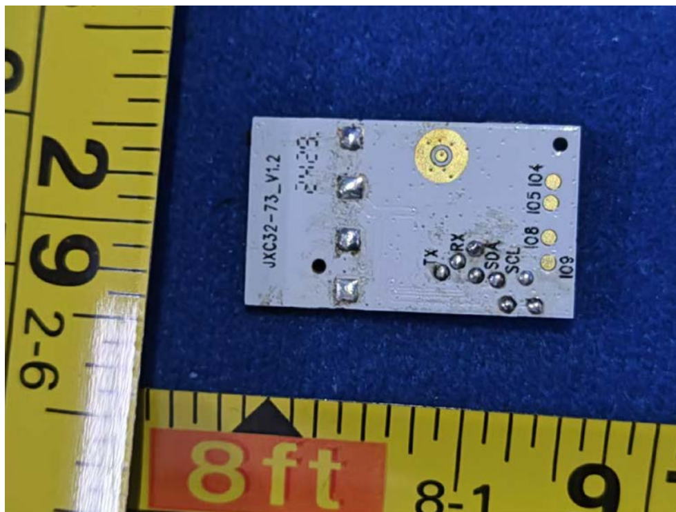
FIGURE 12 DIRECT CONNECT FULL COLOR BR30 (M/N: CLEDR309CD1MS) CHIP & CRYSTAL
