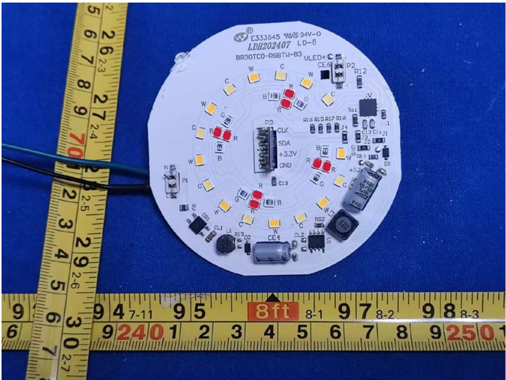
FIGURE 8 DIRECT CONNECT FULL COLOR BR30 (M/N: CLEDR309CD1MS) MAINBOARD FRONT
