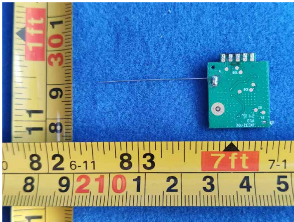
FIGURE 12 DIRECT CONNECT FULL COLOR A21 (M/N: CLEDA2116CDMS) CHIP&CRYSTAL ON BOARD
