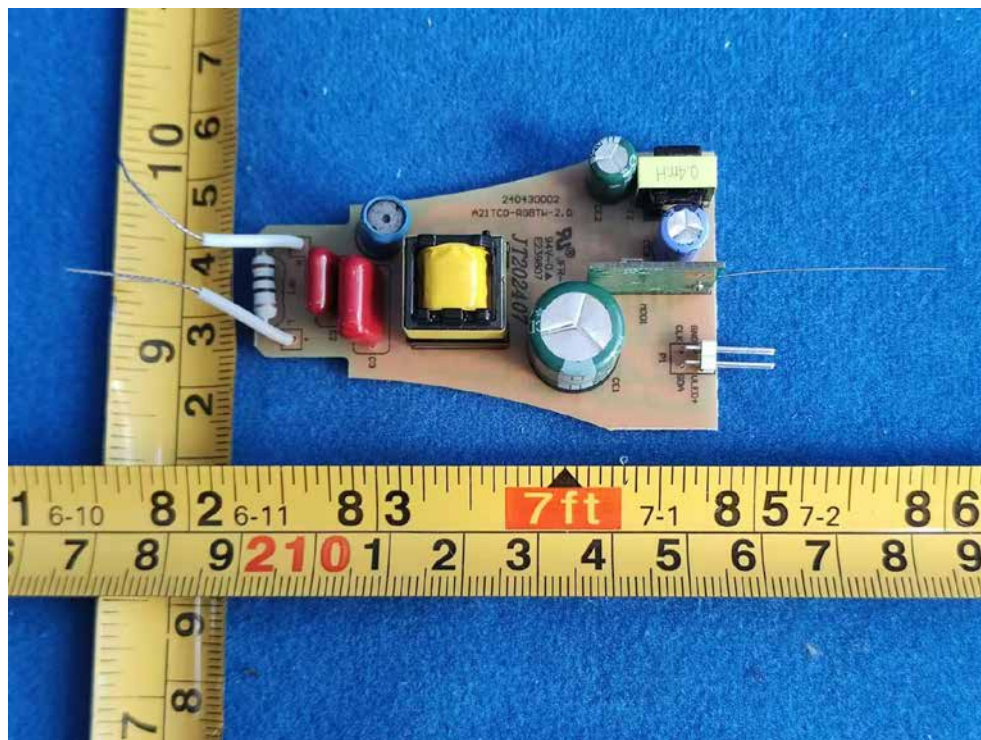
FIGURE 8 DIRECT CONNECT FULL COLOR A21 (M/N: CLEDA2116CDMS) MAINBOARD FRONT
