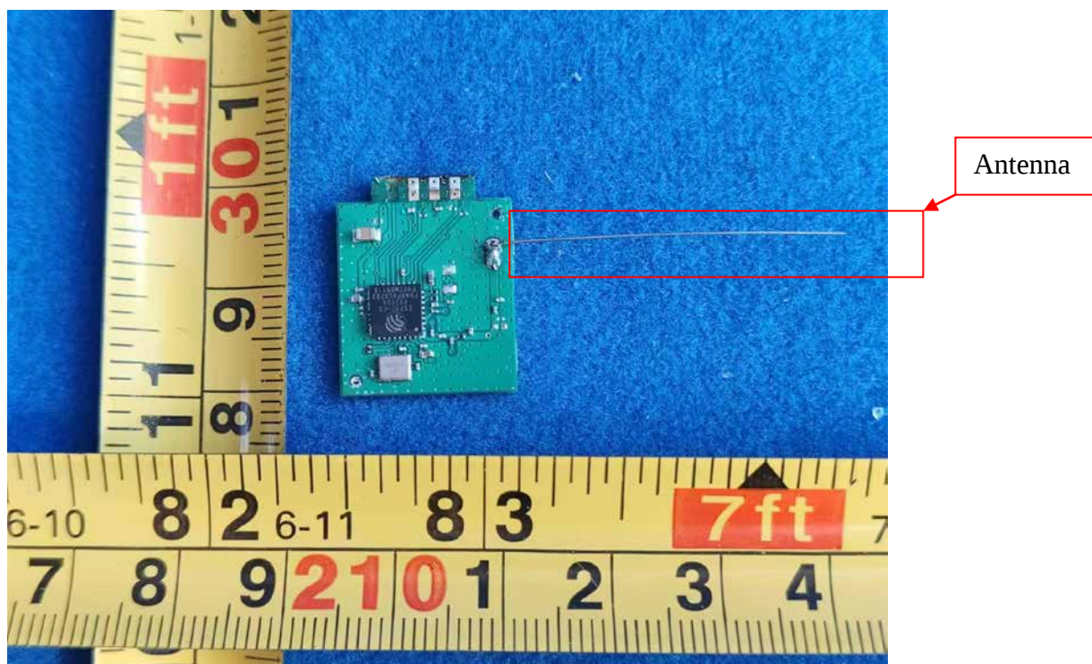
FIGURE 10 DIRECT CONNECT FULL COLOR A21 (M/N: CLEDA2116CDMS) RF BOARD FRONT
