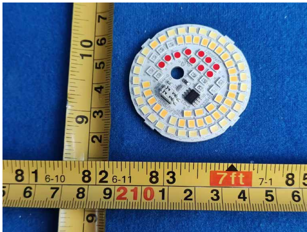
FIGURE 14 DIRECT CONNECT FULL COLOR A21 (M/N: CLEDA2116CDMS) LED BACK
