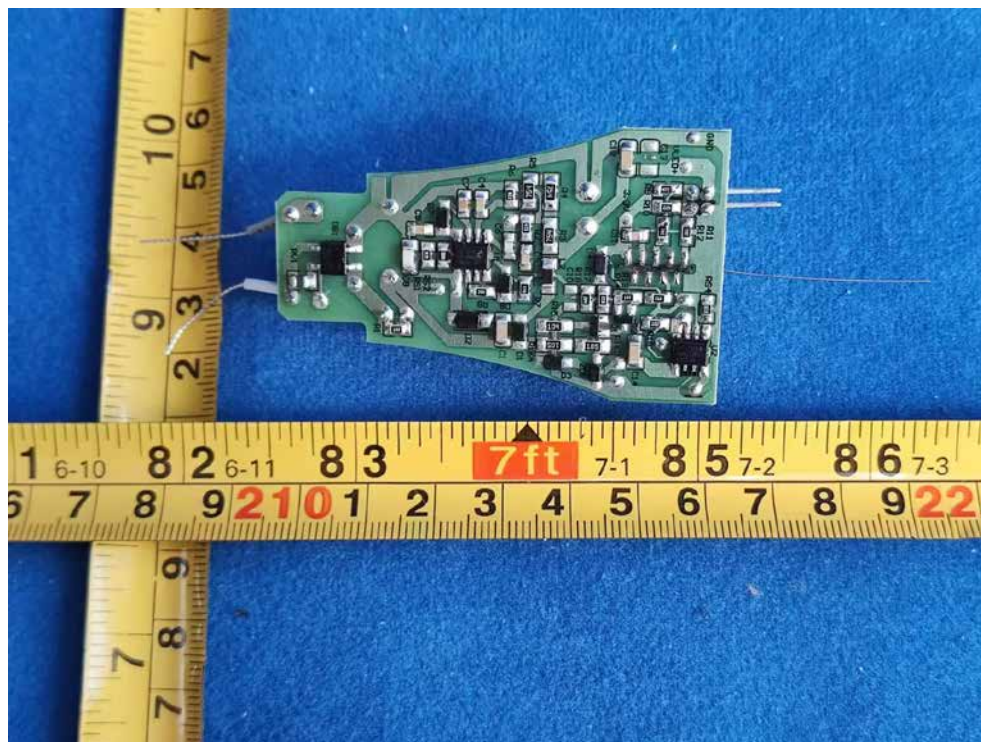
FIGURE 10 DIRECT CONNECT FULL COLOR A21 (M/N: CLEDA2116CDMS) RF BOARD FRONT
